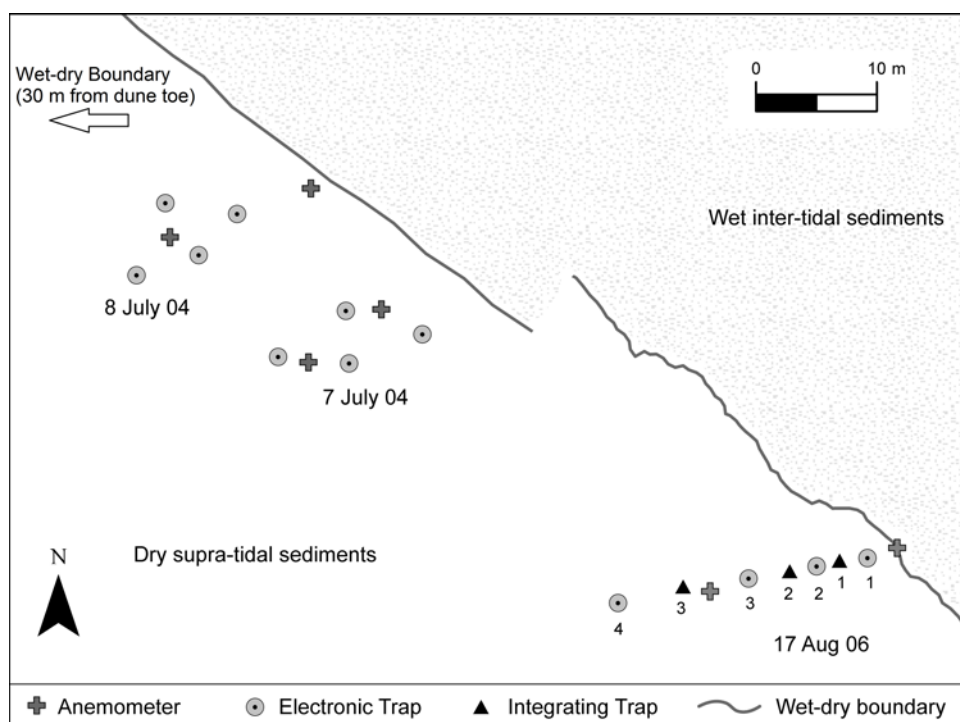
Figure 2. Instrument locations.
