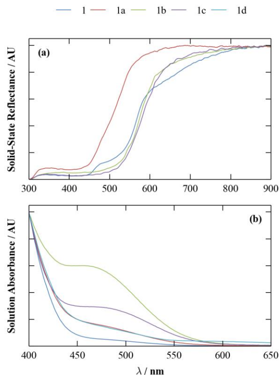
Fig. 4 Optical properties of Lawsonsone ( 1 ) and its cocrystals with 4,4'-bipyridine ( 1a ), 4-(2-pyridine-4-ethyl)pyridine ( 1b ), 1,3-di(4-pyridyl)propane ( 1c ) and 2-hydroxy pyridine ( 1d ). The two plots show the normalised solid-state reflectance spectra of 1 and 1a-1c (a), and the solution absorbance spectra of 1 and 1a-1d (b), recorded in the wavelength range 300-900 and 400-650 nm, respectively. To better identify the position of the transition edges in the reflectance spectra, the first derivatives were calculated by numerical differentiation (see supporting information).
