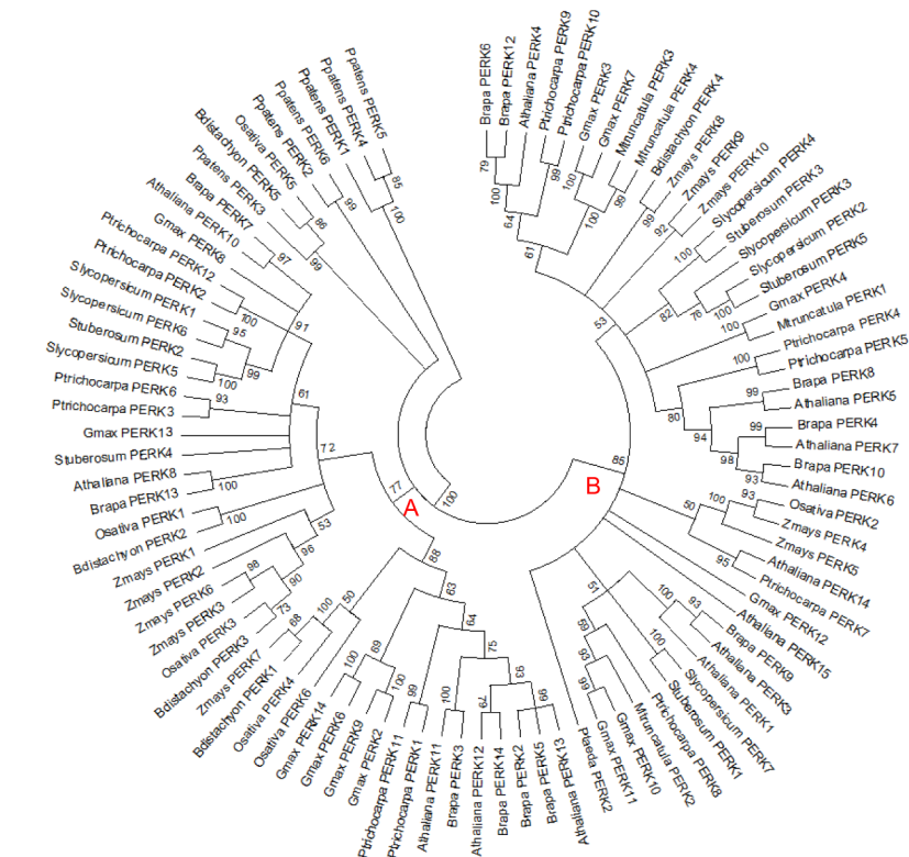
Fig 7. Maximum Likelihood Analysis of PERKs. The evolutionary history was inferred by using the Maximum Likelihood method based on the JTT matrix-based model. The bootstrap consensus tree inferred from 1000 replicates is taken to represent the evolutionary history of the taxa analyzed. Branches corresponding to partitions reproduced in less than 50% bootstrap replicates are collapsed. The analysis involved 93 amino acid sequences. There were a total of 283 positions in the final dataset. A and B represent two major clades.
