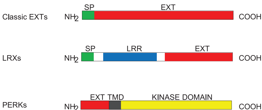
Fig 5. Structural schemes of classical EXTs, LRX, and PERKs. Classical EXTs have an N-terminal signal peptide (green) followed only by EXT domain (red). LRXs have an N-terminal signal peptide (green) followed by a leucine-rich region (LRR, blue). The EXT domain (red) of LRXs is located at the C terminus. The EXT domain of PERKs is located at N terminus followed by a transmembrane domain (TMD, black) and a kinase domain (yellow).
