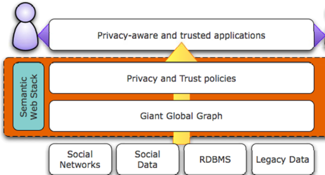
Figure 1: Semantic Web stack for Trust and Privacy on the Social Web
