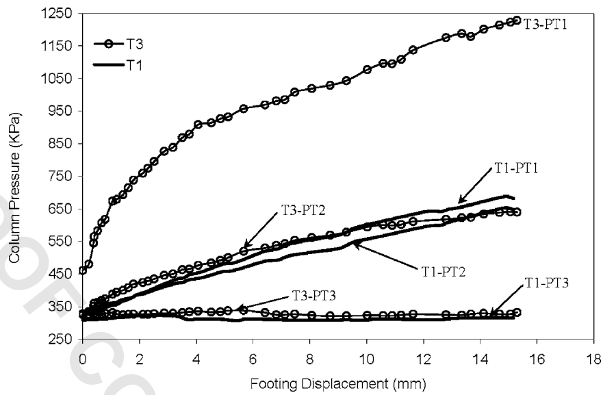
FIG. 8—Pressures read by PT1, PT2, and PT3 during foundation loading.
