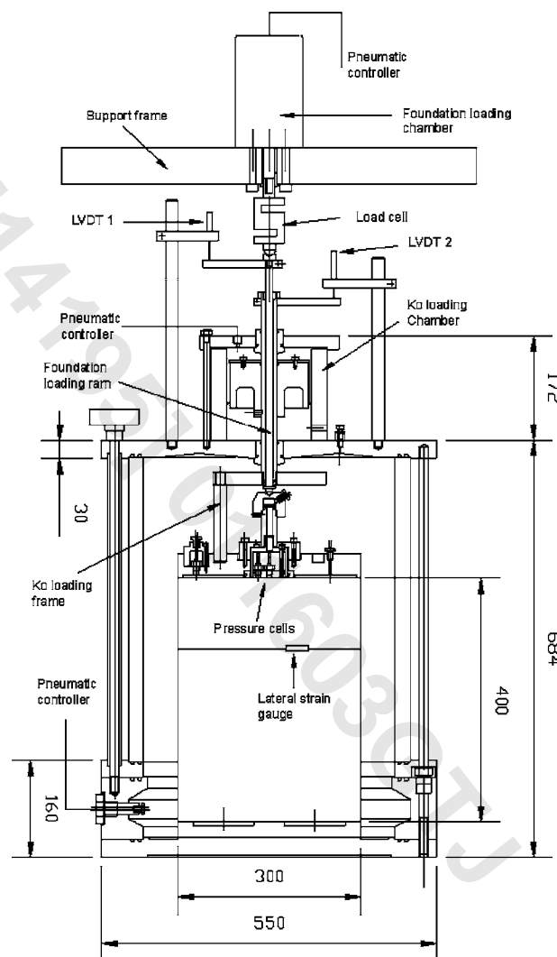
FIG. 3—Sectional view of the test setup (not to scale).
