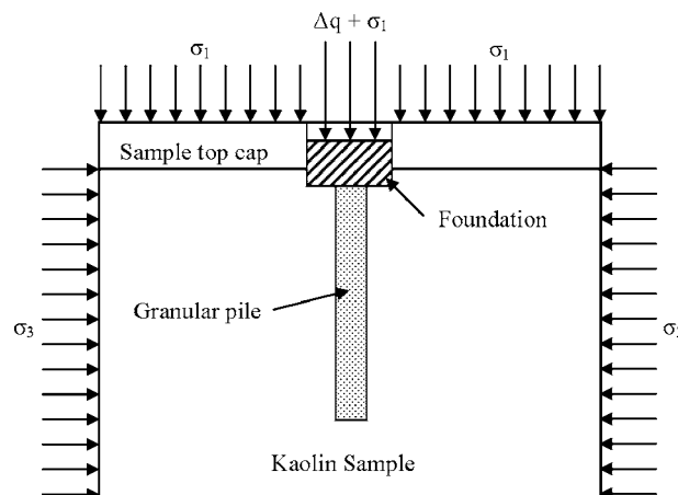
FIG. 2—Proposed loading configuration and test setup.
