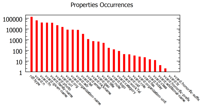
Fig. 3: Properties occurrences in training data (note the logarithmic scale).
