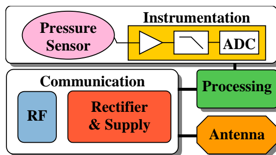
Figure 2. Electronics Synoptic of Endocom
