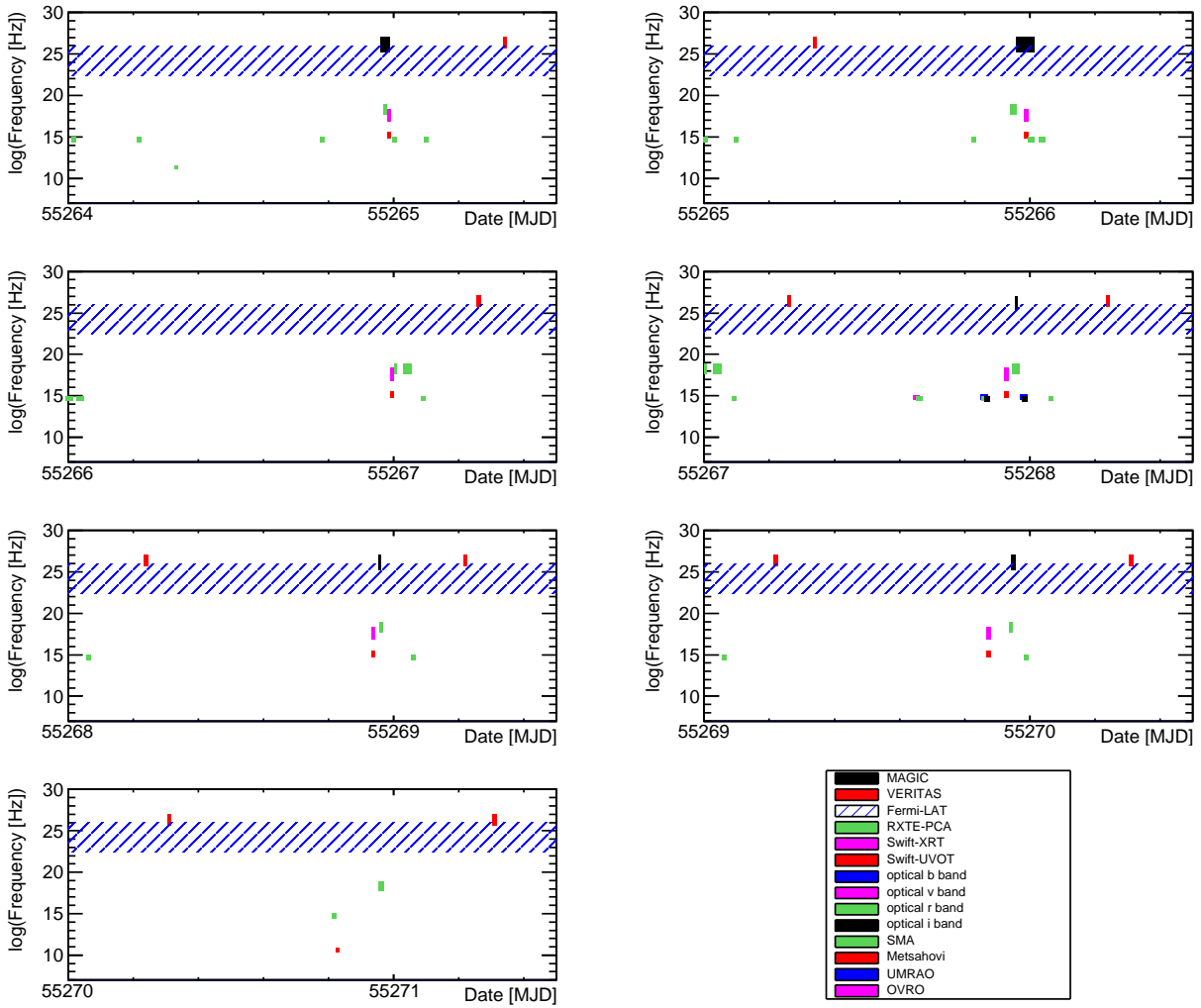
Fig. A.1: Temporal and energy coverage during the flaring activity from 2010 March 10 (MJD 55265) to 2010 March 16 (MJD 55271). Fermi -LAT data were accumulated during two-day time intervals to ensure significant detections of Mrk 421, and is depicted here with a blue band. For better visibility of the observations at UV, optical, and radio band, where the observation time is usually short and the covered frequency band is narrow, an additional 20 minutes in time and half a decade in frequency are included when displaying the results. The names of all the optical instruments are listed in Table 1.
