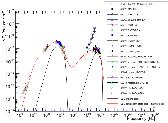
(e) MJD 55270.
