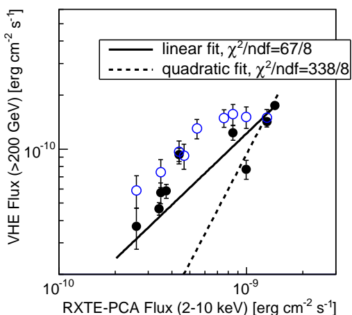
Fig. 4: Correlation between VHE \gamma -ray flux (MAGIC, black solid circles, and VERITAS, blue empty circles) and X-ray fluxes. Top: X-ray flux at the 0.3–2 keV band measured with Swift -XRT. Middle: X-ray flux at the 2–10 keV band measured with Swift -XRT. Bottom: X-ray flux at the 2–10 keV band measured with RXTE -PCA. The lines show the fits with linear and quadratic functions. Only MAGIC data points were used for the fits to ensure VHE-X-ray simultaneity (see Appendix A).
