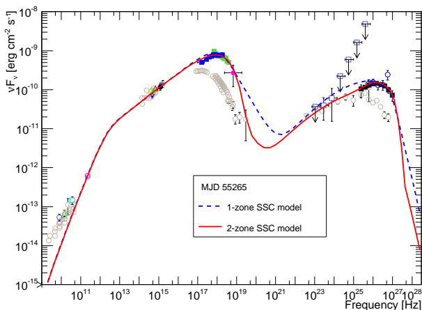
(a) MJD 55265.
