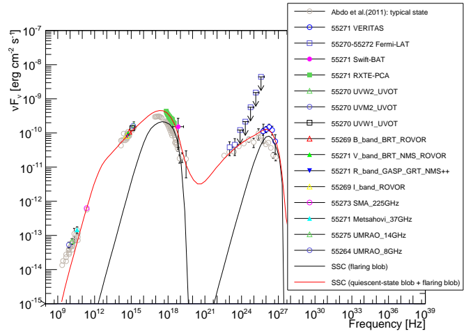
(f) MJD 55271.
