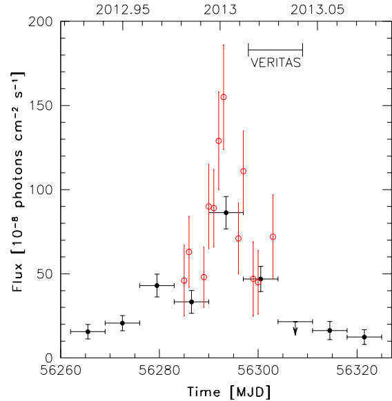
Figure 1. Integrated flux light curve of PMN J0948+0022 obtained by Fermi -LAT in the 0.1–100 GeV energy range during 2012 December 1–2013 January 31 with 7-day time bins. Arrow refers to 2\sigma upper limits on the source flux. Upper limits are computed when TS < 10 . Open circles represent daily fluxes reported for the periods of high activity. No upper limits are shown for daily data. The horizontal line indicates the period of the VERITAS observation.
