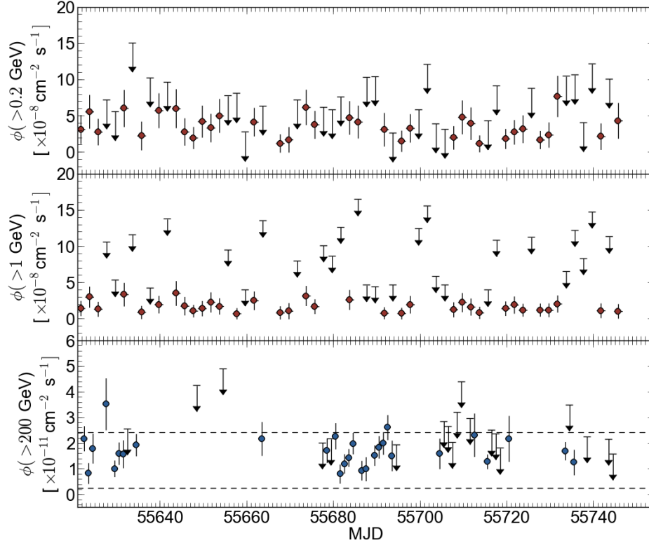
Fig. 4.— Fermi -LAT PG 1553+113 bi-daily flux light curve (2011) above 200 MeV (upper plot) and 1 GeV (middle plot), in units of \text{cm}^{-2} \text{s}^{-1} , for the time periods contemporaneous with VERITAS observations, and VERITAS daily integral flux light curve above 200 GeV (lower plot), in units of \text{cm}^{-2} \text{s}^{-1} . The upper and lower dashed lines indicate the integral fluxes above 200 GeV corresponding to 10% and 1% of the Crab Nebula flux, respectively. The black arrows represent 2\sigma upper limits.
