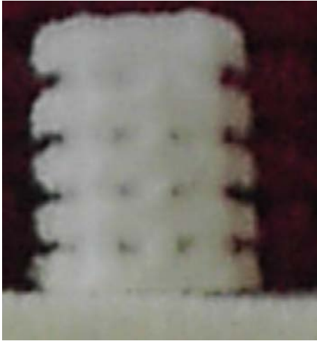
Fig. 4 a) Side view of PCL compressive sample, b) top view of PCL compressive sample.
