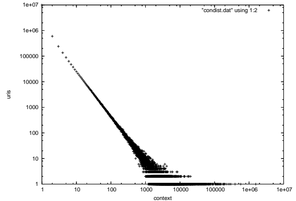
Figure 3: Number of URIs against the number of contexts they appear in (log/log scale)
