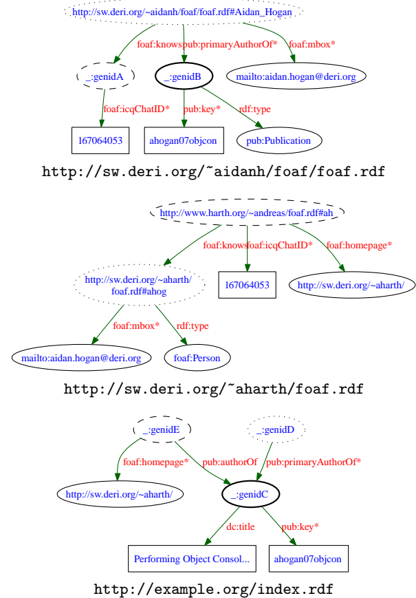
Figure 1: Three sample data graphs from three different sources. Inverse functional properties are depicted with an asterisk (*). Identifiers denoting the same entity are denoted by a common line style.
