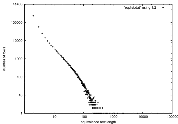
Figure 4: Equivalence row distribution (log/log scale)
