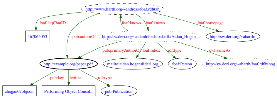
Figure 2: Output of the object consolidation algorithm applied to the three graphs from Figure 1.
