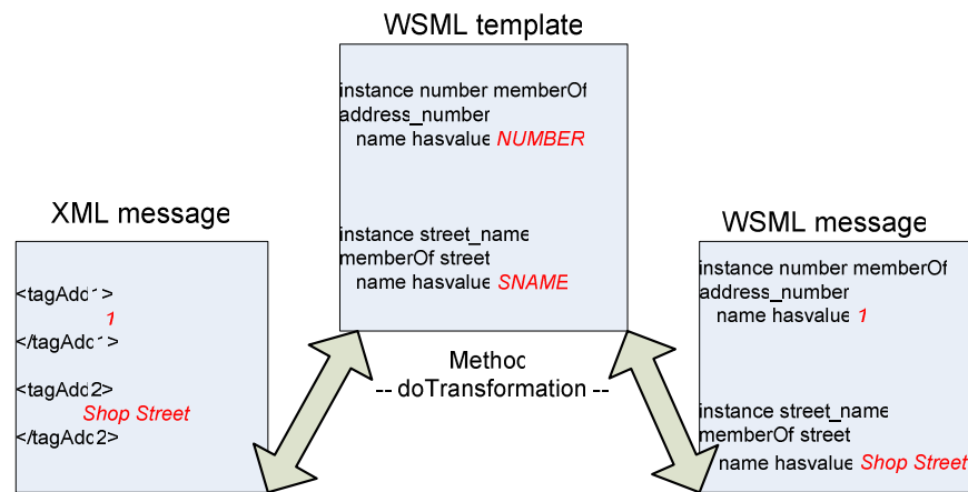
Fig.1. XML to WSMX Transformation.
