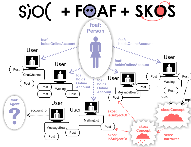
Fig. 2. Combining SIOC, FOAF and SKOS
