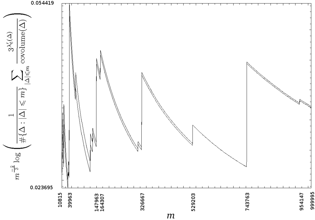
FIGURE 5. Average homological 3-torsion outside subgroups of type \mathcal{D}_3 , scaled as indicated.
