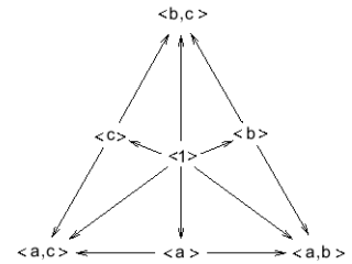
FIGURE 1. Quotient of the Davis complex for a triangle group (diagram reprinted with the kind permission of Sanchez-Garcia [26]).
