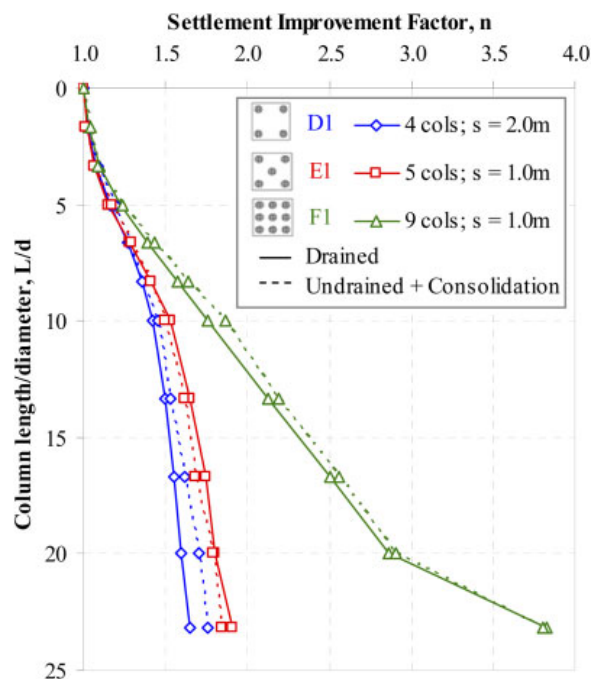
Figure 2. Influence of column length, arrangement and drainage analysis type upon settlement performance of stone columns.
