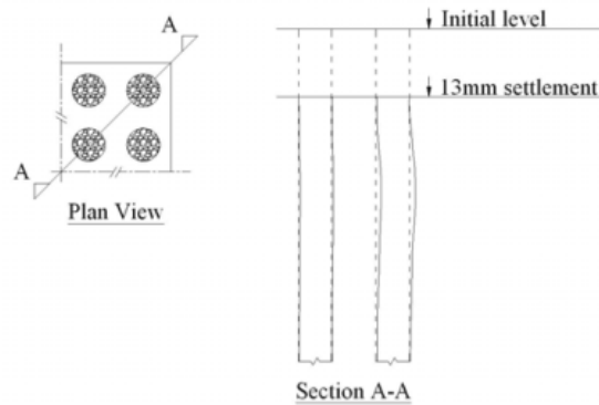
Figure 6. Mode of deformation for 4\text{ m} \times 4\text{ m} group G.
