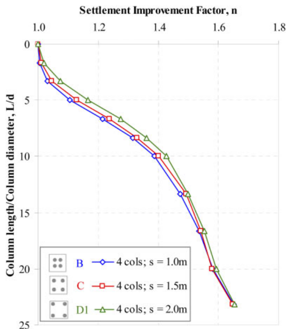
Figure 3. Effect of column spacing (or position in relation to the edge of the footing) on settlement performance.
