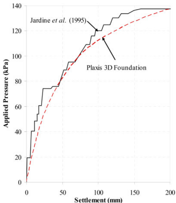
Figure 1. Validation of soil profile and parameters for a footing on untreated Carse clay.
