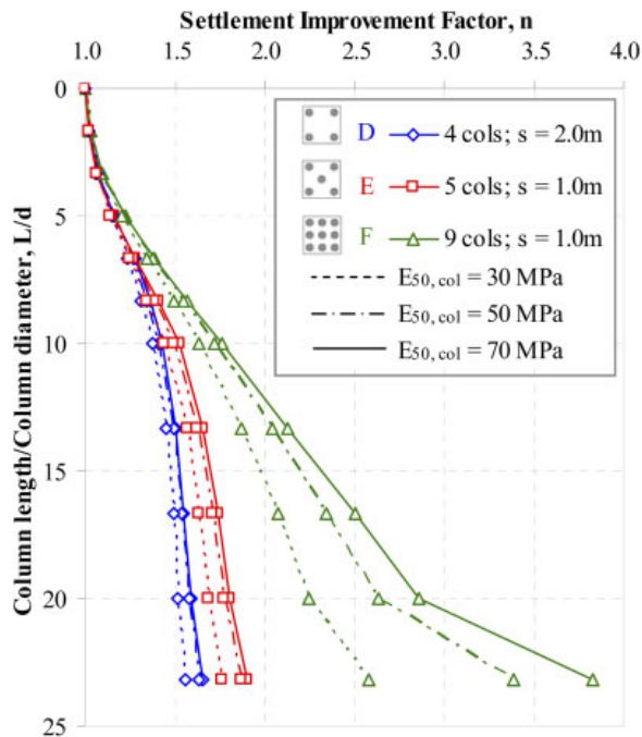
Figure 4. Effect of column stiffness upon settlement performance.
