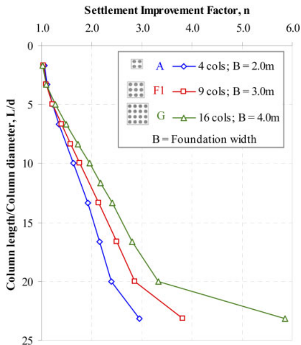
Figure 5. Effect of column confinement upon settlement performance.
