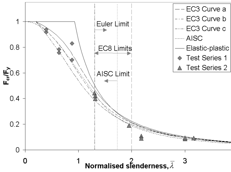
Figure 6. Normalised buckling loads of cyclic specimens.
