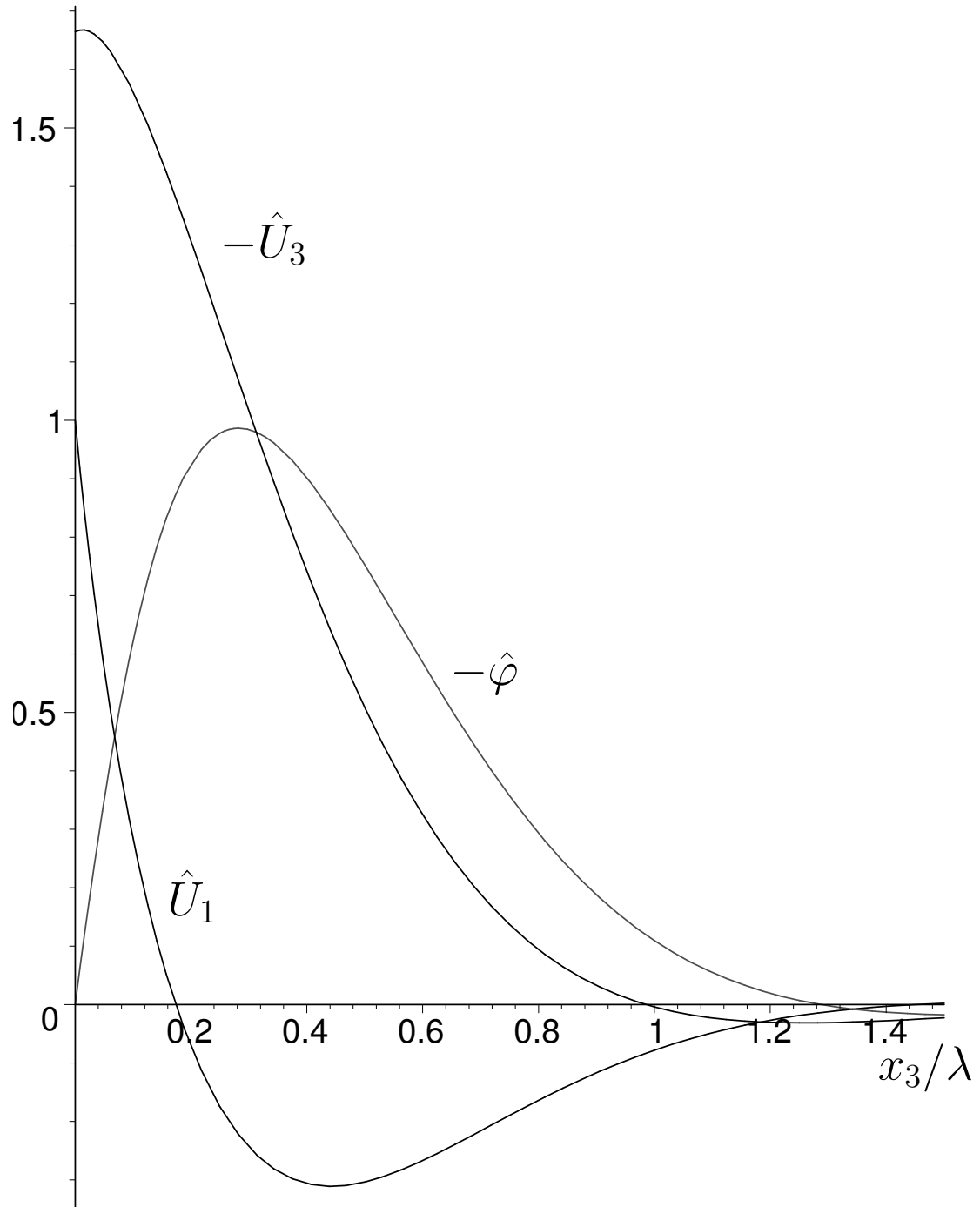
Figure 1: Depth profiles of the mechanical displacements ( \text{\AA} ) and the electric potential (V) for the piezoelectric Rayleigh wave in \text{KNbO}_3 , Z-cut X-propagation with metallized boundary conditions.
