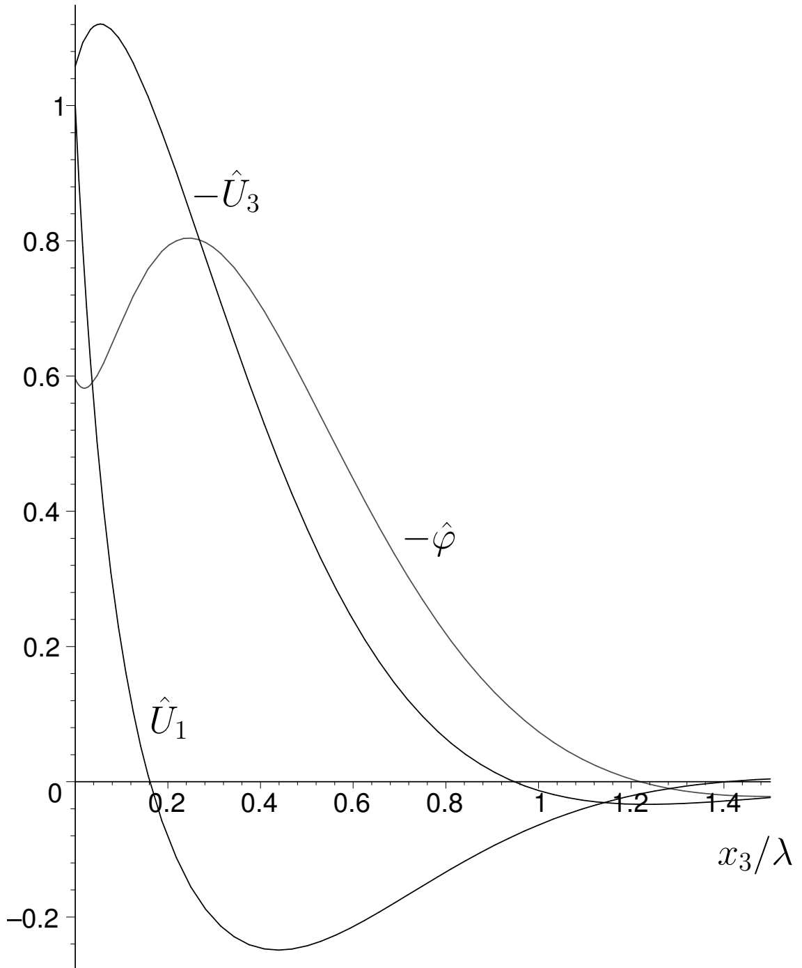
Figure 2: Depth profiles of the mechanical displacements ( \text{\AA} ) and the electric potential (V) for the piezoelectric Rayleigh wave in \text{KNbO}_3 , Z -cut X -propagation with unmetallized boundary conditions.
