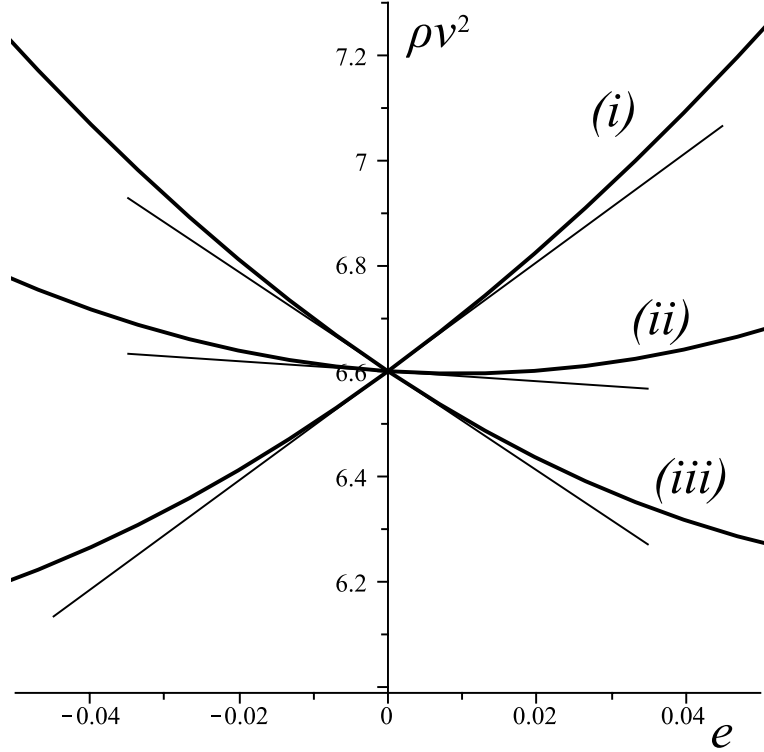
Figure 2: Shear bulk waves propagating in a uni-axially deformed incompressible block: \rho v^2 (in kPa) against the elongation e in the case of waves traveling (i) in the x_1 -direction (then, all shear waves travel with speed given by Eq.(12), irrespective of the direction of polarization); (ii) in any direction in the (x_1, x_2) -plane or in the (x_1, x_3) -plane, with transverse polarization in that plane, and speed given by Eq.(13); (iii) in any direction in the (x_1, x_2) -plane or in the (x_1, x_3) -plane, with polarization normal to that plane, and speed given by Eq.(14). The thin straight lines correspond to the linear part of the \rho v^2 - e curves. Here the initial shear modulus is \mu = 6.6 kPa, the third-order Landau constant is A = -37.7 kPa, and the coefficient of non-linearity is \nu = 3.5 , in line with the experimental results of Renier et al.[6].
