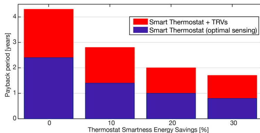
Figure 8. Payback period analysis of proposed retrofit solutions as a function of the energy savings produced by thermostat smartness.
