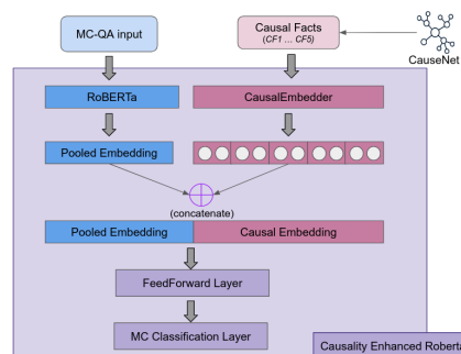
Figure 2: Architecture of Causality Enhanced RoBERTa. The architecture takes as input the multiple-choice question input and relevant causal facts selected from CauseNet.
