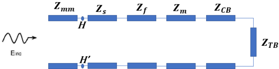
Fig. 3 The transmission line model of 1-D heel structure. The Z_{mm} , Z_{HH'} , Z_s , Z_f , Z_m , Z_{CB} , and Z_{TB} represent impedance of matching medium, plane HH' , skin, fat, muscle, cortical bone, and trabecular bone respectively
