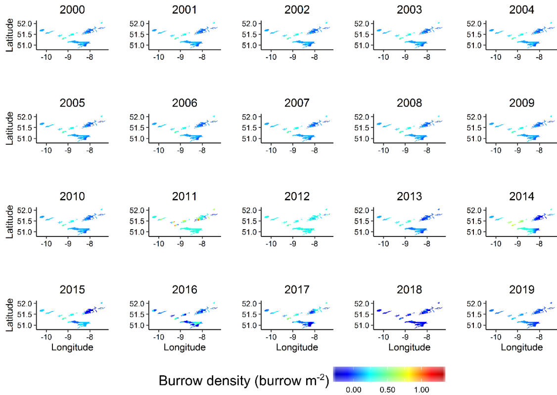
Figure A4. Spatial distribution of N. norvegicus burrow densities from underwater TV survey on the South Coast (FU19) grounds. Initial horizontal distribution of particles was based on spatial distribution of burrows, whereby higher proportions of particles were released from areas of the grounds with higher burrow densities. Please note number of particles remained constant (10,000). For years that burrow distribution data were unavailable, an average distribution of available years was used (2000 - 2010).
