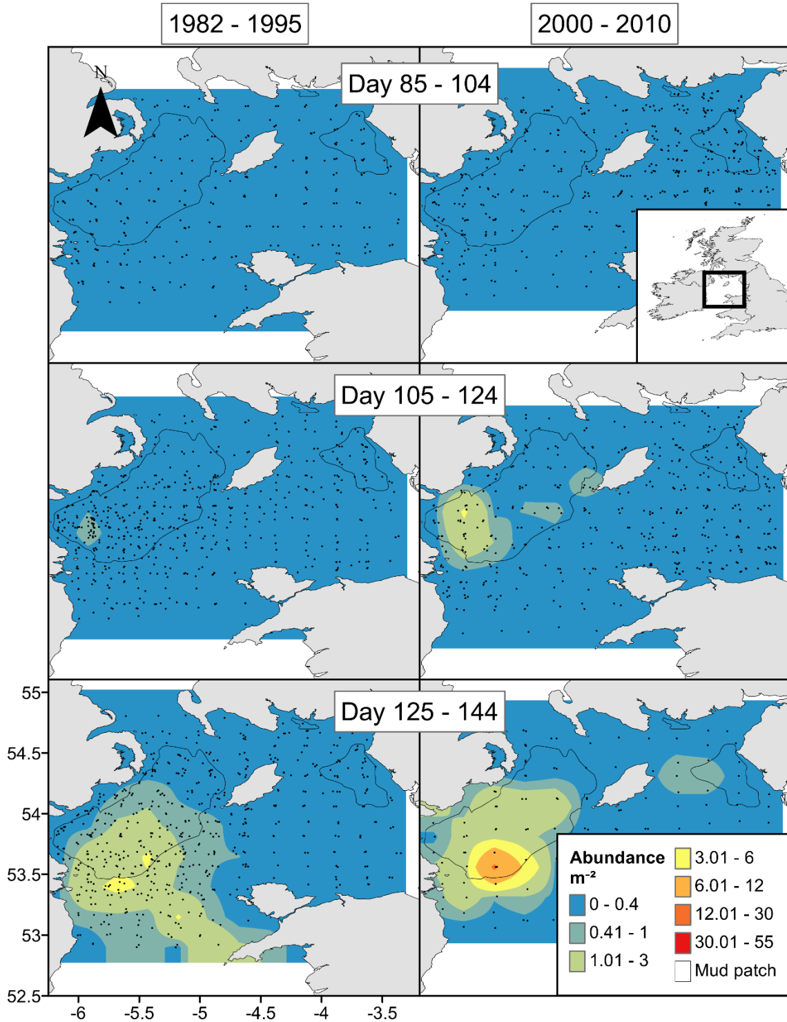
Figure A3. Comparison of Stage III N. norvegicus larval abundance m^{-2} in the Irish Sea during the time series 1982 - 1995 and 2000 - 2010 at distinct Day of Year (DOY) time periods. Black markers indicate the position of each station and inverse distance weighted spatial interpolation is used. Nephrops norvegicus grounds for both western and eastern Irish Sea are indicated by the continuous black line.
