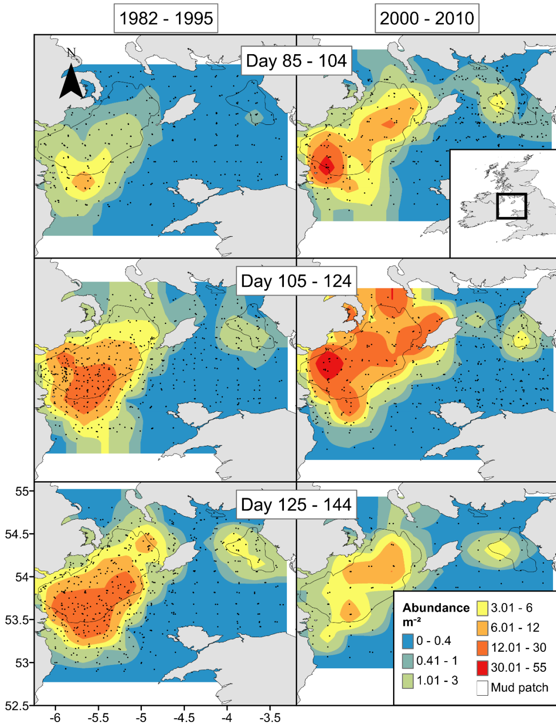
Figure 5. Comparison of Stage I N. norvegicus larval abundance m^{-2} in the Irish Sea during the time series 1982 - 1995 and 2000 - 2010 at distinct Day of Year (DOY) time periods. Black markers indicate the position of each sampling station and inverse distance weighted spatial interpolation is used. Nephrops norvegicus grounds for both western and eastern Irish Sea are indicated by the continuous black line.
