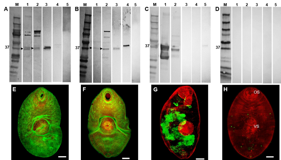
Fig 5. Immune detection of native F. hepatica serpins. (A–D) Western blot analysis of somatic extracts of F. hepatica NEJ 24 hr post-excystment and adult parasites and the recombinant F. hepatica serpins FhSrp1 and FhSrp2. Lane 1: NEJ 24 hr somatic extract (30 µg/lane); lane 2: adult worm somatic extract (30 µg/lane); lane 3: recombinant rFhSrp1 (0.1 µg/lane); lane 4: recombinant rFhSrp2 (0.1 µg/lane); lane 5: recombinant rFhCL3 (0.1 µg/lane). Immunoblots were probed with (A) anti-rFhSrp1 polyclonal antibodies raised in rabbit, (B) anti-rFhSrp2 polyclonal antibodies raised in rabbit, (C) anti-rFhCL3 polyclonal antibodies raised in rabbit or (D) rabbit pre-immune serum as a negative control. M: molecular weight. (E–H) Whole mount NEJ 24 hr post-excystment immunolocalisation of the F. hepatica serpins by confocal laser microscopy represented by green fluorescence (FITC staining). (E) Fixed NEJ probed with anti-rFhSrp1 polyclonal antibodies raised in rabbit. (F) Fixed NEJ probed with anti-rFhSrp2 polyclonal antibodies raised in rabbit. (G) Fixed NEJ probed with anti-rFhCL3 polyclonal antibodies raised in rabbit. (H) Fixed NEJ probed with rabbit pre-immune anti-serum as a negative control. All samples were counter-stained with phalloidin-TRITC to stain muscle tissue (red fluorescence). OS, oral sucker. VS, ventral sucker. Scale bars, 20 µM.
