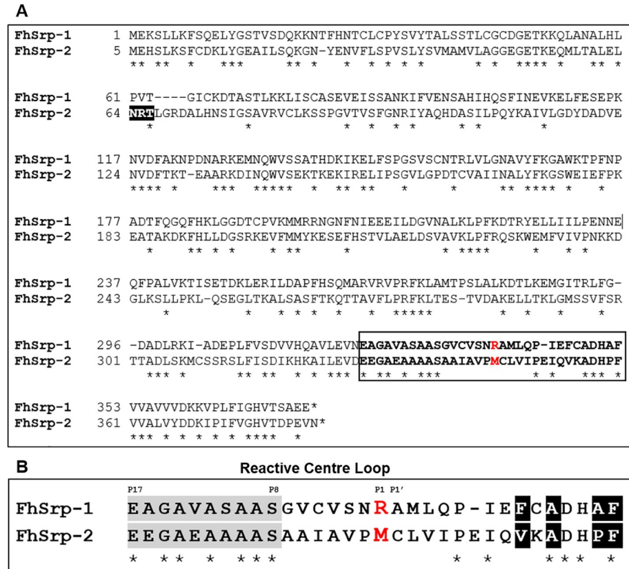
Fig 3. Comparative analysis of F. hepatica serpin 1 and 2 proteins. (A) Clustal Omega alignment of the FhSrp1 and FhSrp2 protein sequences. The reactive centre loop region (RCL) is boxed and the predicted P1 residue is highlighted in red. The putative N-glycosylation site is highlighted in black. (B) Alignment of the RCL sequences. The residues within the conserved hinge region, P17–P8, are shaded in grey, the predicted P1 position is in red and the amino acids predicted to form the shutter region (PROSITE signature PS00284) are highlighted in black. Asterisks below the alignment indicate residues identical in the two serpins.
