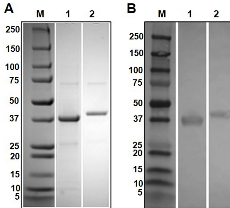
Fig 4. Recombinant expression of F. hepatica serpins. (A) rFhSrp1 (lane 1) and rFhSrp2 (lane 2) expressed in E. coli BL21 cells, purified by affinity column, resolved in a 4–20% SDS-PAGE gel and stained with Biosafe Coomassie; (B) rFhSrp1 (lane 1) and rFhSrp2 (lane 2) at 1 \mu g/lane were electro transferred onto a nitrocellulose membrane and probed with the mouse monoclonal antibody to poly-histidine (1:10,000). M: molecular weight in kDa (Precision Plus Protein Dual, Bio-Rad).
