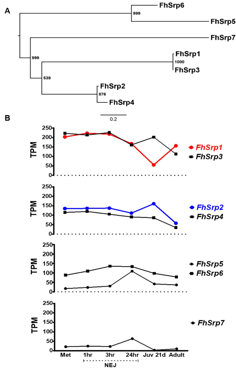
Fig 2. Phylogenetic analysis and gene transcription of the Fasciola hepatica serpin family. (A) Midpoint-rooted maximum likelihood phylogram generated by PhyML based on the protein sequence Arg 224 -Glu 374 (FhSrp1 nomenclature) that includes the reactive centre loop (RCL) region. Bootstrap support values (1000 iterations) are shown at each node. (B) Graphical schematic of the relative gene expression for F. hepatica serpin family represented by transcripts per million (TPM) during the parasite's lifecycle within the mammalian host: the infective metacercariae (Met), newly excysted juveniles (NEJ) at 1 hr, 3 hr and 24 hr post-excystment, liver stage juvenile parasites 21-days post infection (Juv 21d) and bile duct stage mature adult parasites (Adult). The serpin genes, FhSrp1 and FhSrp2 chosen for further characterisation are highlighted in red and blue, respectively.
