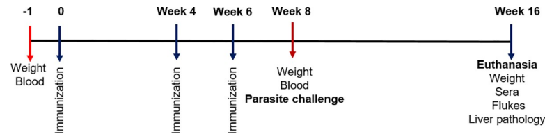
Fig 1. Graphical schematic showing the schedule for the F. hepatica serpin vaccine trial in rats. Red arrows show when the blood samples were taken.
