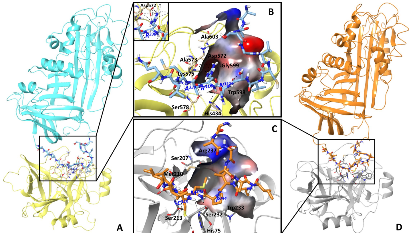
Fig 8. Molecular homology modelling of FhSpr1-kallikrein and FhSpr2-chymotrypsin complexes. The homology models of FhSpr1 and FhSpr2 were built based on Manduca sexta serpin 1B (PDB code: 1K9O), whereas the structures of kallikrein and chymotrypsin were rebuilt from the corresponding crystal structures of these enzymes with PDB codes, 1CBW and 5TJX, respectively. The protein-protein complexes were obtained via the protein structure alignment to the serpin-trypsin complex (PDB code: 1K9O). (A) Overall structure of the FhSpr1-kallikrein complex is shown in the cyan and yellow cartoons, respectively. (D) Overall structure of the FhSpr2-chymotrypsin complex is shown in the orange and grey cartoons, respectively. (B) and (C) Zoomed in views of the FhSpr1 and FhSpr2 serpin reactive centre loop (RCL) within the active site of the kallikrein and chymotrypsin serine proteases, respectively. The interacting residues of the serine proteases and the serpin RCL are visualized in stick-like representation. The P1 pocket and the linked area are shown as surface-like representations coloured with the electrostatic potential. Hydrogen bonds and a salt bridge are highlighted in black. Residue labels for kallikrein and chymotrypsin are shown in black and in blue for FhSpr1 and FhSpr2. In the FhSpr1-kallikrein complex (B) the R 338 residue of FhSpr1 is within the narrow negatively charged S1 pocket that forms the salt bridge interaction with Asp 572 and hydrogen bonds with the backbone of Gly 599 , Ala 603 and Ala 573 . The polar interactions between the Arg 338 and Asp 572 residues are shown in the insertion image. In the FhSpr2-chymotrypsin complex (C), the M 345 residue of FhSpr2 sits closely within the spacious uncharged S1 pocket forming many Van der Waals interactions with the residues of the pocket that collectively contribute to the overall tight binding.
