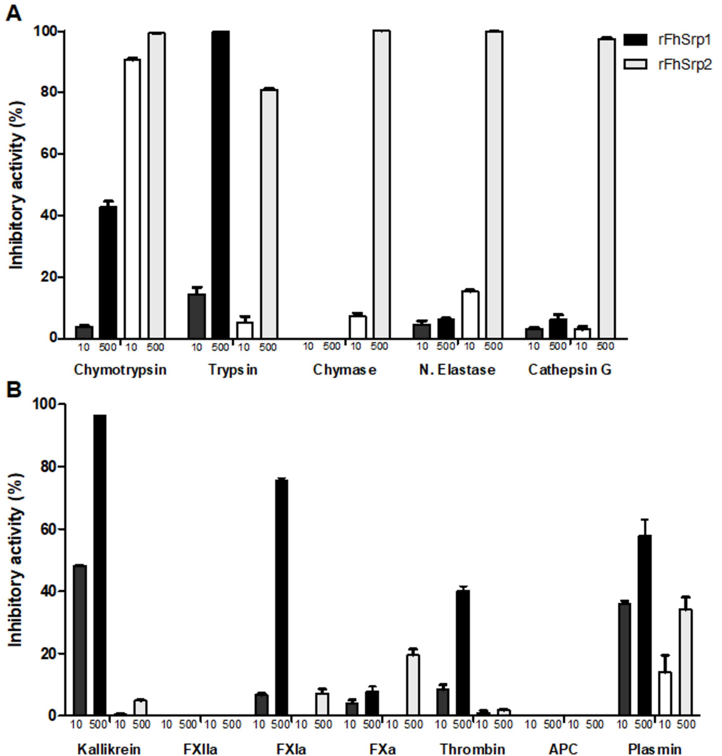
Fig 6. Inhibitory activity of F. hepatica serpins against a panel of serine proteases involved in (A) digestion and host defence, and (B) coagulation. The activity of chymotrypsin (4.0 nM), trypsin (168 nM), chymase (0.6 μM), neutrophil elastase (50 nM), cathepsin G (100 nM), kallikrein (150 nM), FXIIa (7.6 nM), FXIa (3.68 nM), FXa (5.8 nM), thrombin (800 pM), activated protein C (APC) (0.5 μM) and plasmin (800 μM) were tested in the presence of 10 and 500 nM rFhSrp1 (dark bars) or rFhSrp2 (light bars). Inhibition is presented relative to the activity of each enzyme in the absence of inhibitors and error bars indicate standard deviation of three separate experiments.
