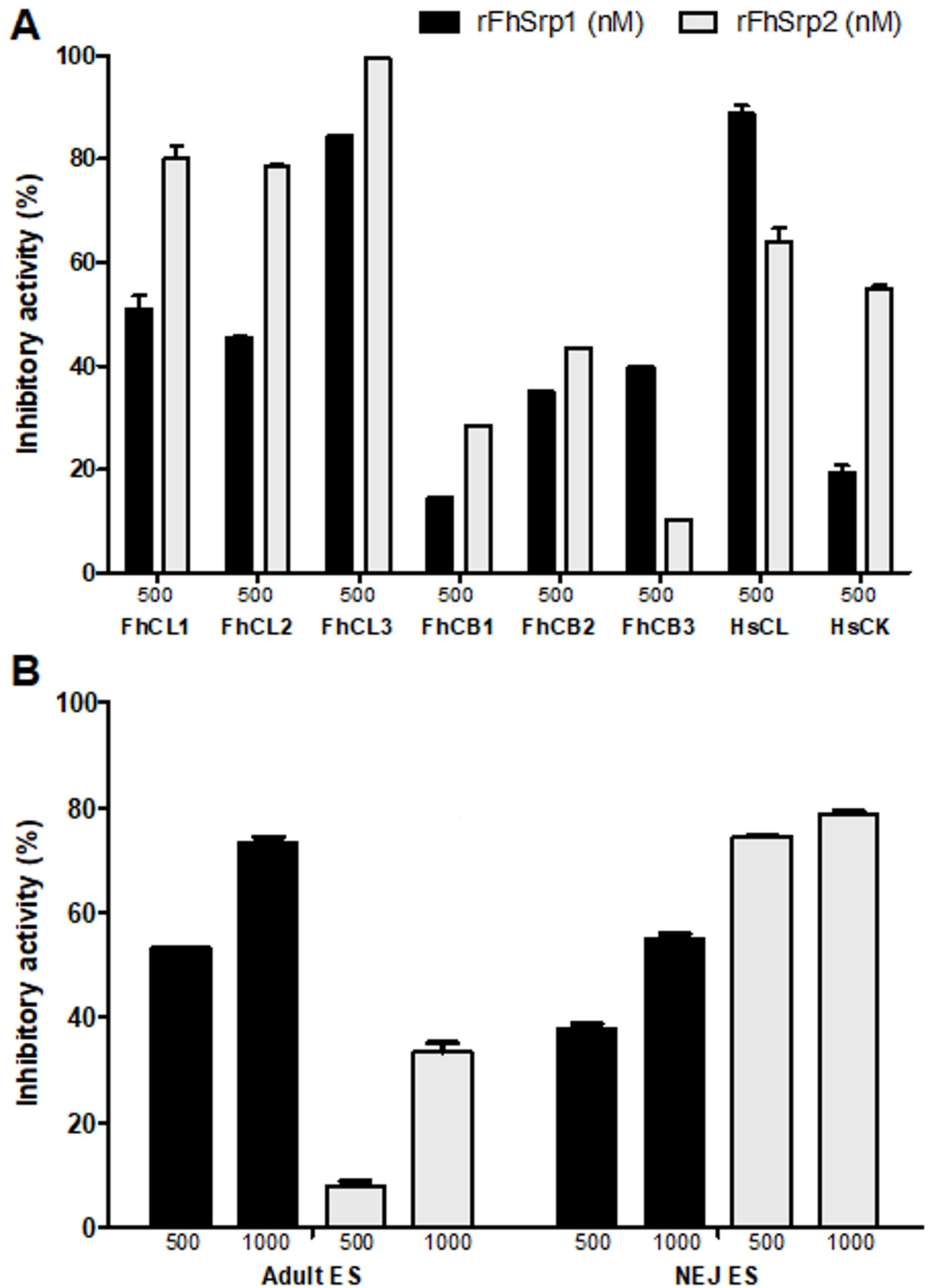
Fig 9. F. hepatica serpins inhibit parasite and host cysteine proteases. The activity of F. hepatica cathepsin cysteine proteases, FhCL1 (2.7 nM), FhCL2 (5.0 nM), FhCL3 (5.0 nM), FhCB1 (135 nM), FhCB2 (270 nM), FhCB3 (135 nM), and human cathepsin cysteine
