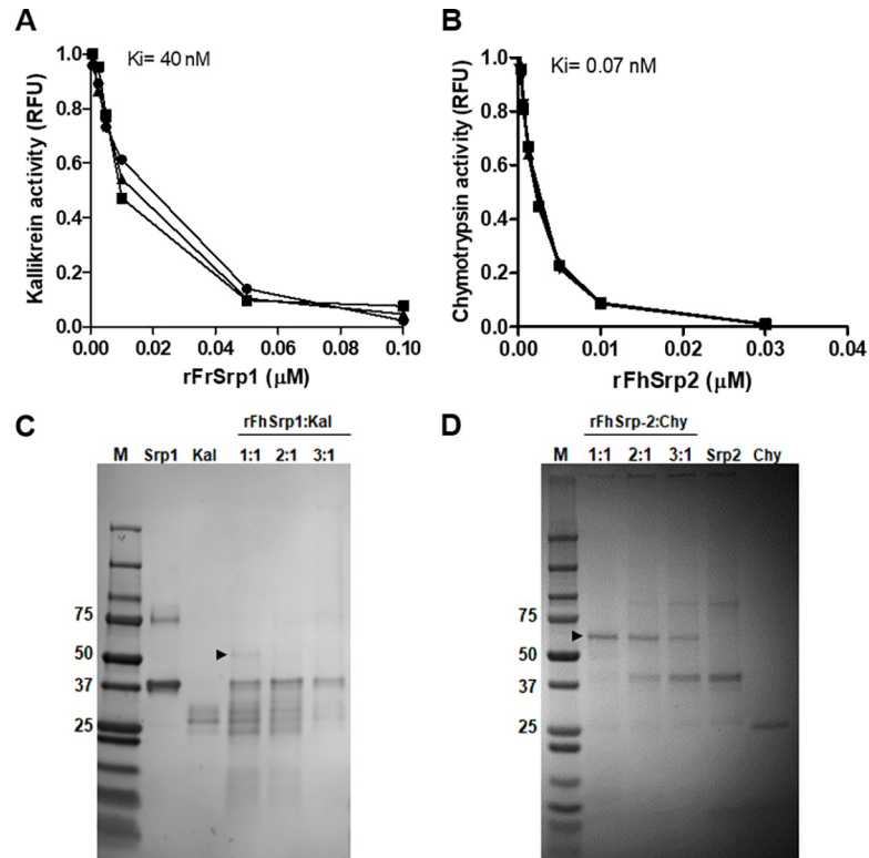
Fig 7. hepatica serpins inhibit specific serine proteases by forming covalent complexes. F. (A) Inhibition constant ( K_i ) of kallikrein as a function of rFhSrp1 concentration. (B) Inhibition constant ( K_i ) of chymotrypsin as a function of rFhSrp2 concentration. The curves represent the best fit to the Morrison equation (C) Serpin/serine protease complex formation between rFhSrp1 (Srp1) and kallikrein (Kal) was analyzed by SDS-PAGE under non-reducing conditions at serpin/protease ratios of 1:1, 2:1 and 3:1. Covalent complex formation occurs at ~55 kDa (black arrowhead) (D) Serpin/serine protease complex formation between rFhSrp2 (Srp2) and chymotrypsin (Chy) was analyzed by SDS-PAGE under non-reducing conditions at serpin/protease ratios of 1:1, 2:1 and 3:1. Covalent complex formation occurs at ~60 kDa (black arrowhead). Molecular weight (M) in kDa.
