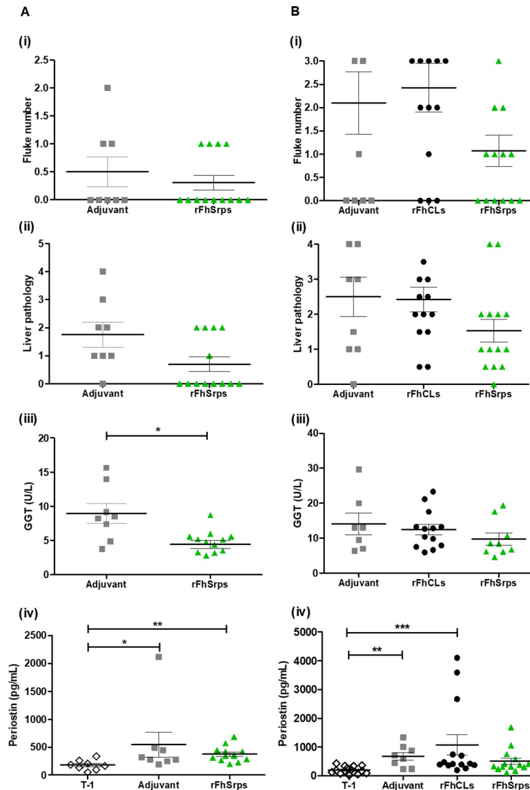
Fig 11. Evaluation of F. hepatica serpins as vaccine candidates. Results are presented for each trial individually, on the left the first trial (A) and on the right the second trial (B), representing the adjuvant control group (Adjuvant), the animals vaccinated with the F. hepatica recombinant cathepsin L2 and cathepsin L3 proteases (FhCLs) and the animals vaccinated with the F. hepatica recombinant serpin 1 and 2 (FhSrps). T-1 represents sera samples collected before vaccination at the beginning of the trial. (i) Number of flukes recovered from the bile duct; (ii) Liver pathology, (iii) Gamma-glutamyl transferase (GGT) sera levels and (iv) Periostin sera levels. Error bars indicate standard error of three separate experiments. Statistical differences between groups was assessed by Mann Whitney or One-way Anova followed by Kruskal-Wallis test (95% confidence intervals) ( p < 0.05 : *; p < 0.01 : **; p < 0.001 : ***).
