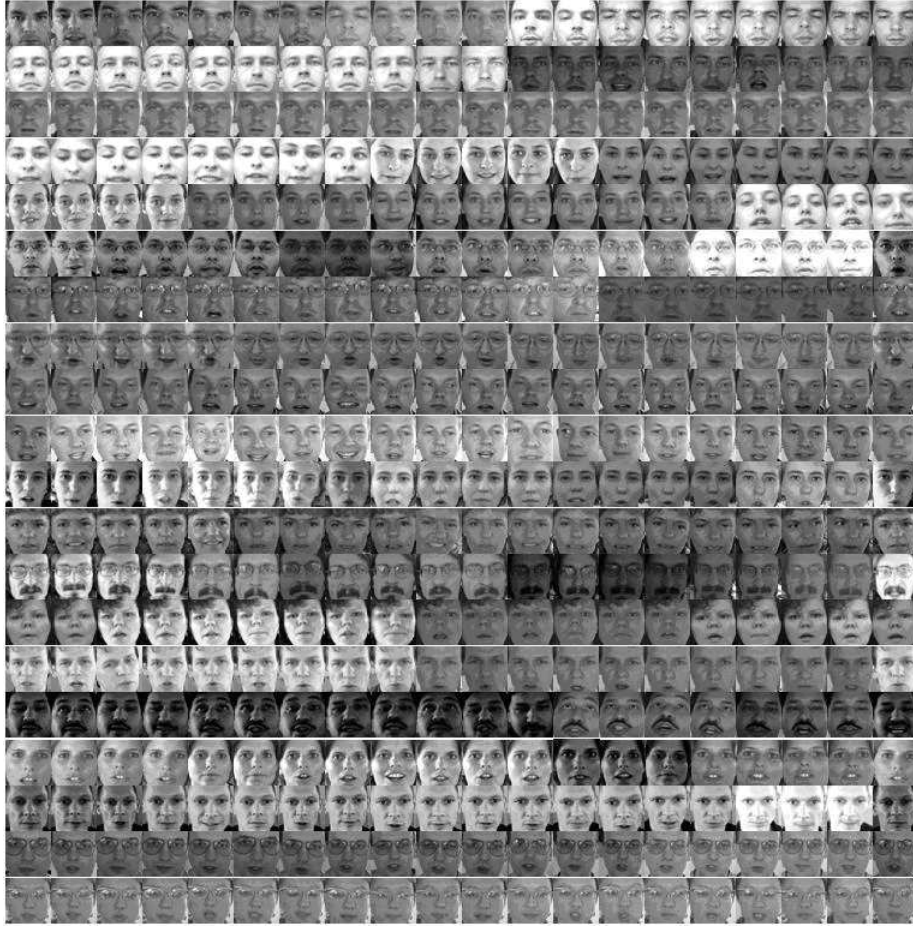
Figure 6.8: BioID database
