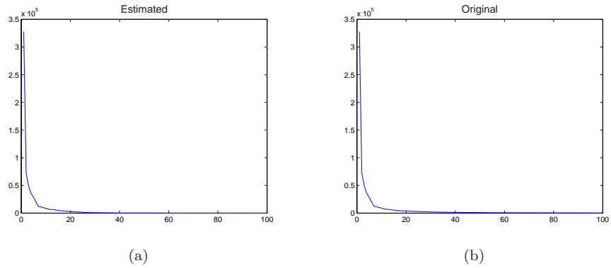
Figure 9.3: Eigenvalue representations a) original and b) estimated
