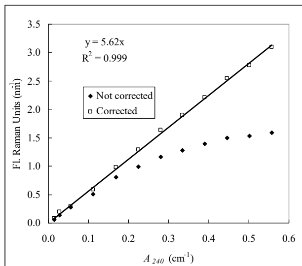
Figure 6: Example of the ability of the inner filter correction procedure to correct for non-linearities between the fluorescence and absorbance of an analyte (in this case Suwannee River Fulvic Acid).
