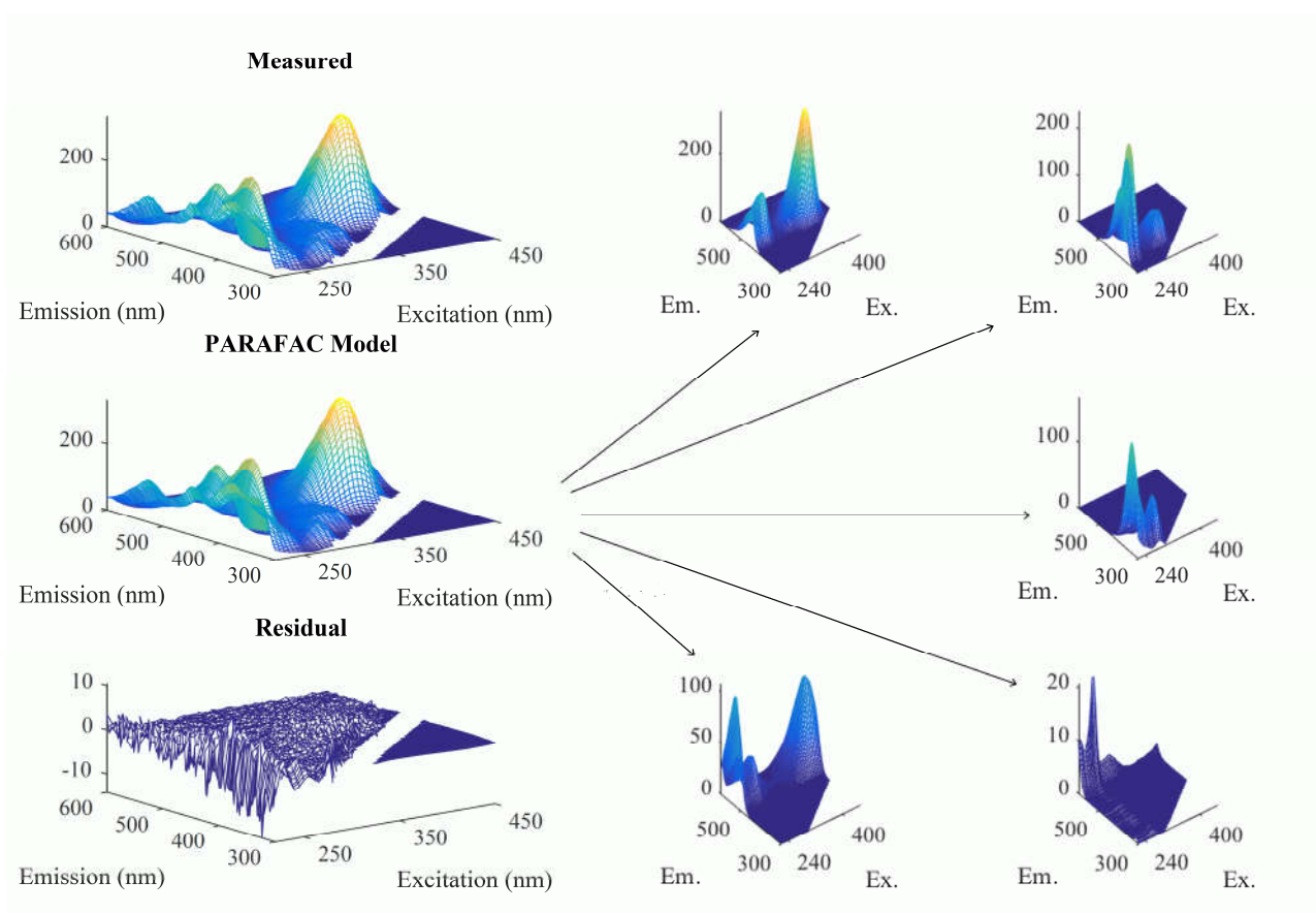
Figure 7: The results of a five component PARAFAC model of a mixed solution of the fluorescence standards. Left: The measured EEM is a mixture of five fluorophores (BAM-F001, BAM-F002, BAM-F003, BAM-F004, BAM-F005). The model is the five-component model derived by PARAFAC. The residual EEM is the unexplained fluorescence signal and represents largely instrumental noise. Right: The 3D representations of the five PARAFAC components which correspond to each of the BAM fluorophores.
