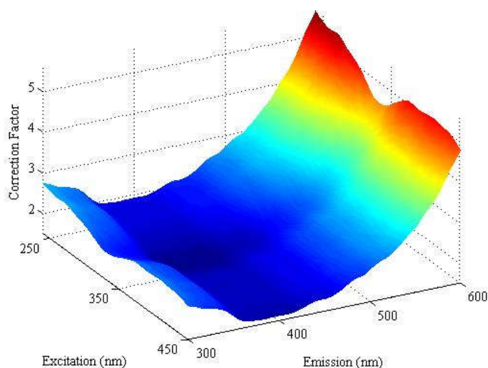
Figure 2: Representative example of an EEM correction factor derived by multiplying the excitation and emission correction factors. A more detailed discussion of the process is included in ref. [25]
