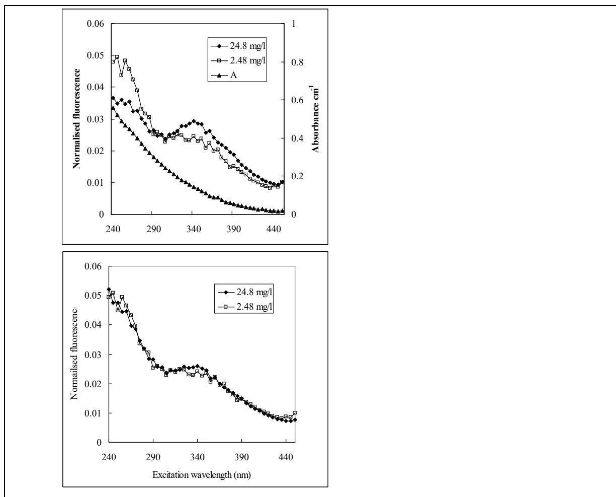
Figure 5: Correcting for inner filter effects. A) Graph of the normalized excitation spectrum of Suwannee River Fulvic Acid at two concentrations. Additionally, the measured UV-Vis absorbance properties are shown (24.8 mg/l). b) The same normalized excitation spectra after correction for inner filter effects using equation 3.
