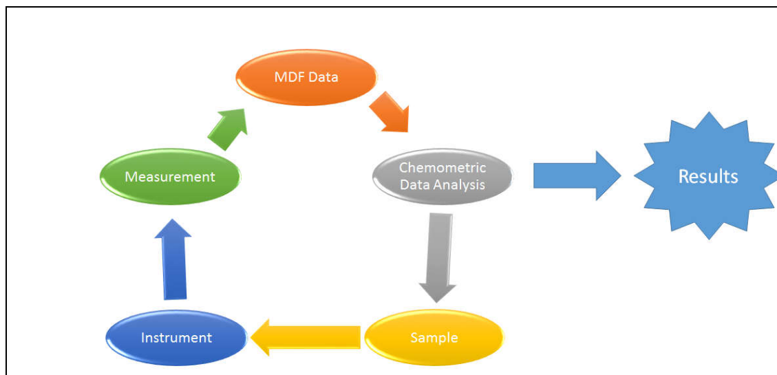
Figure 9: The interlinking nature of the MDF operational cycle as applied to analytical methods. For each element in the cycle (data-instrument-measurement-data-analysis) appropriate controls and procedures need to be implemented to generate accurate and useful output results.
