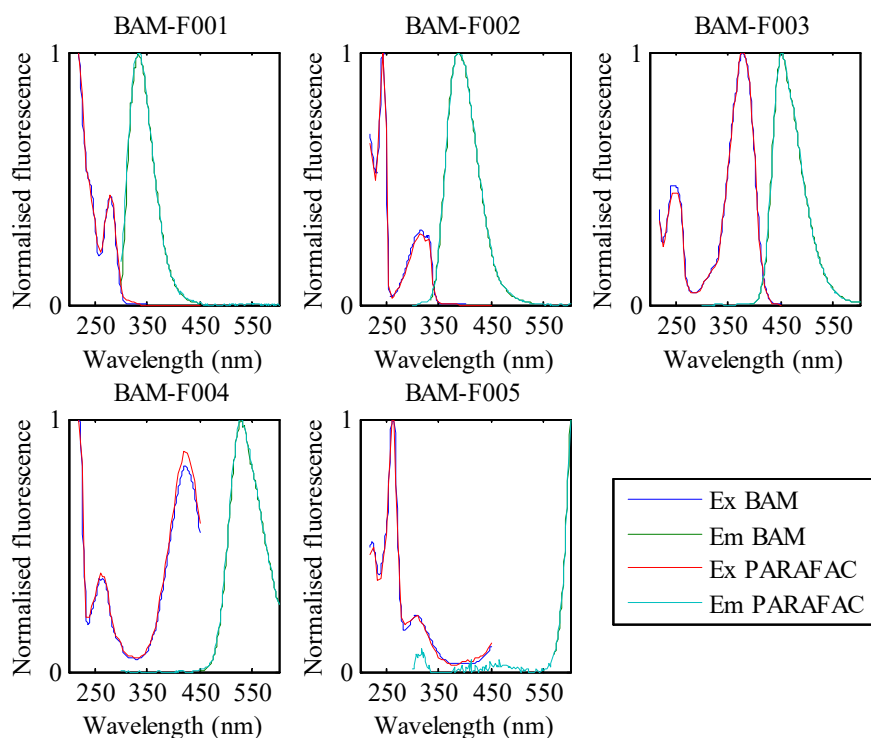
Figure 8: The excitation and emission spectra of the five BAM fluorescence standards measured individually (Ex BAM and Em BAM), plotted together with the five spectral components identified in the PARAFAC model of the mixture (Ex PARAFAC and Em PARAFAC). The emission scans of the pure standards are averages of four replicate scans as required by BAM.
