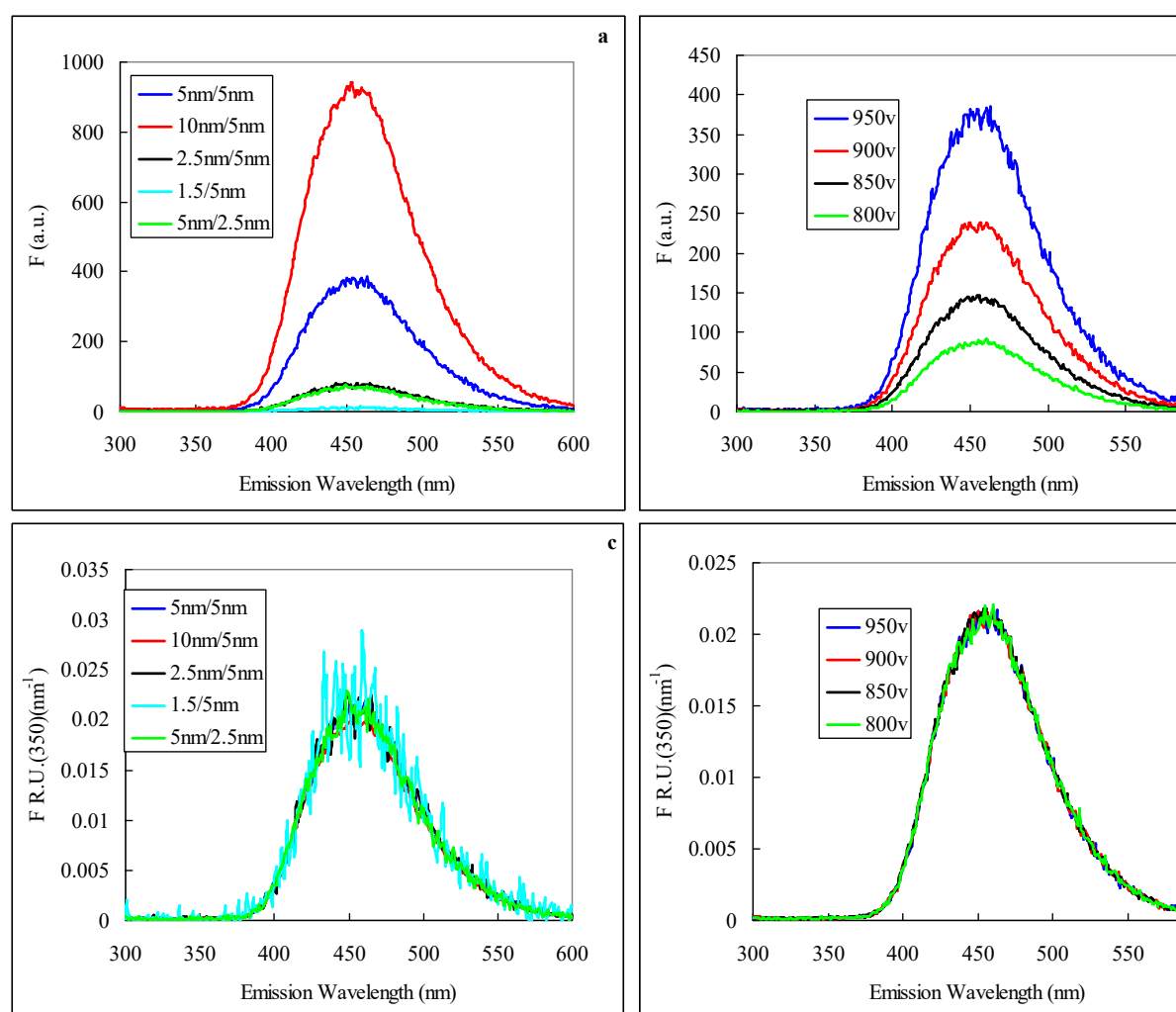
Figure 4: Demonstration of the ability of the Raman quantification approach to remove instrumental set up effects on fluorescence intensity. The emission spectrum of a 5 ppb solution of quinine sulphate is shown measured with a) different excitation and emission slit widths, b) different PMT voltage (detector gain). Plots c) and d) are the same data after Raman quantification relative to the Raman scatter from 350 nm. [32]
