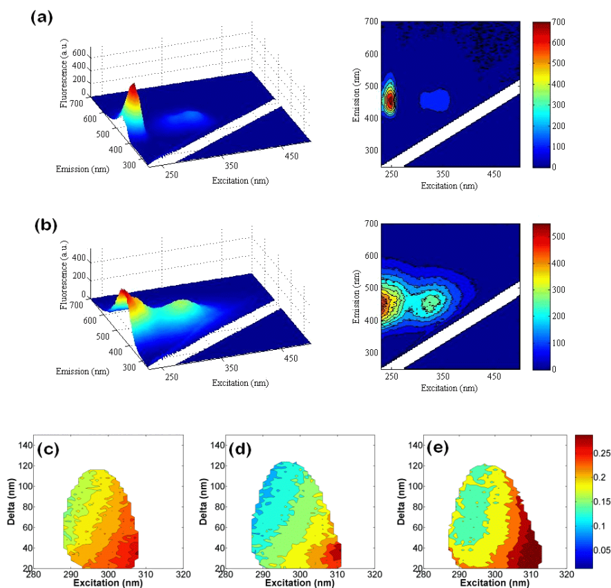
Figure 1: Landscape and contour plots representative of MDF data: a ). EEM of a solution of 50 ppb quinine sulfate in 0.105 M HClO 4 ; b ). EEM of an aqueous solution of Suwannee River Fulvic Acid; c-e ). Changes in the aniso-TSFS contour plots (from ARMES) for Human Serum Albumin (HSA) 1 mg mL -1 in buffer undergoing thermal unfolding: c ) 10 °C, d ) 50 °C, and e ) after cooling from 70 to 20 °C (color scale denotes the anisotropy)[9].
