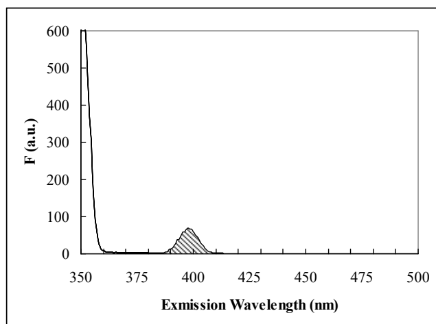
Figure 3: Emission scan of MilliQ water (excitation wavelength 350 nm). The first peak is due to Rayleigh scatter (elastic) and the second to non-elastic Raman scatter (shaded area = A_{rp} ).
