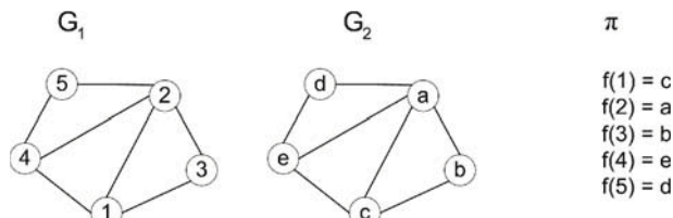
Figure 3: An example of graph isomorphism G_2 = \pi(G_1)
