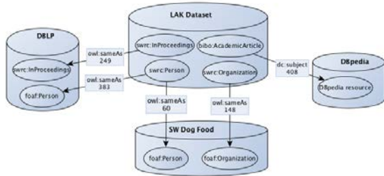
Fig. 2 : Links in the LAK Dataset 28
