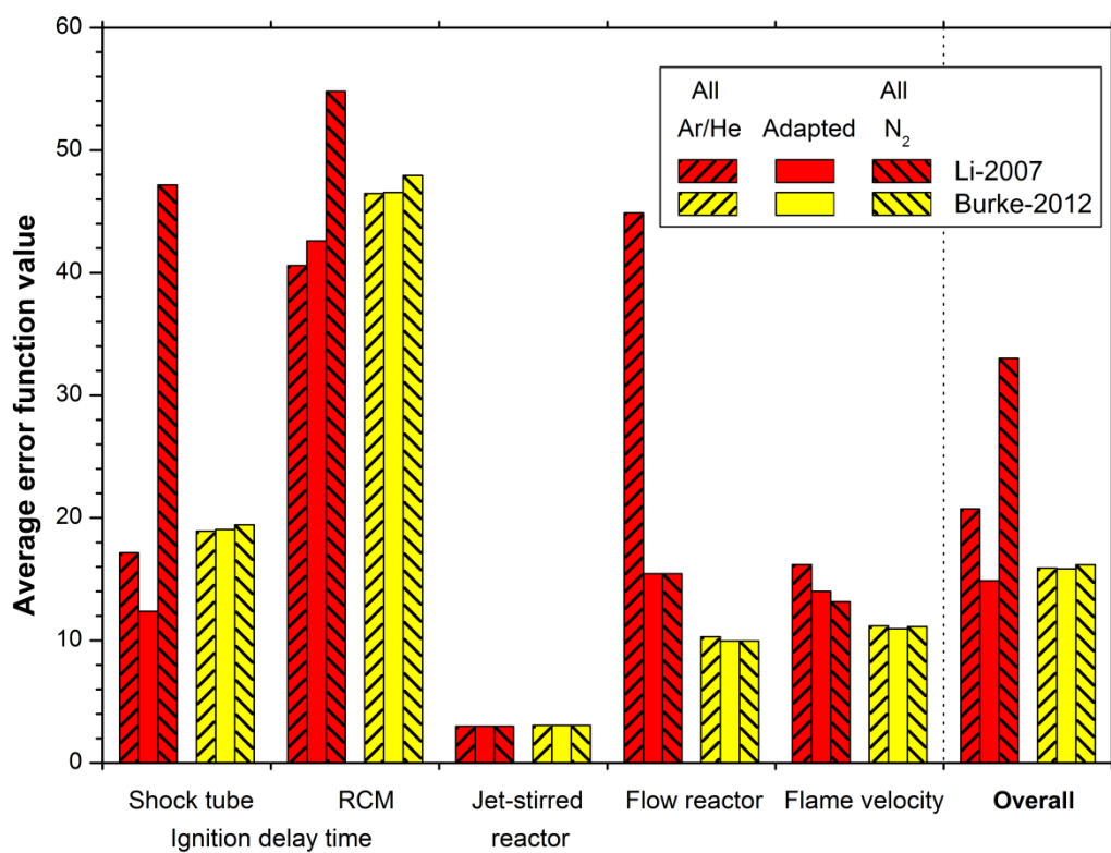
Fig. 12: Comparison of different parameterizations of the reaction \text{H}+\text{O}_2(+\text{M}) = \text{HO}_2(+\text{M}) in the Li-2007 and Burke-2012 mechanisms.
