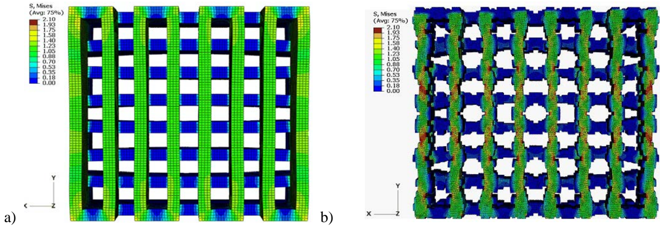
Fig. 9. Contour plot of von Mises stress distribution (MPa) for two scaffolds with exactly the same porosity that were compressed in the y direction. It was found that the effective modulus of the scaffold on the right was 68% higher than that on the left.
