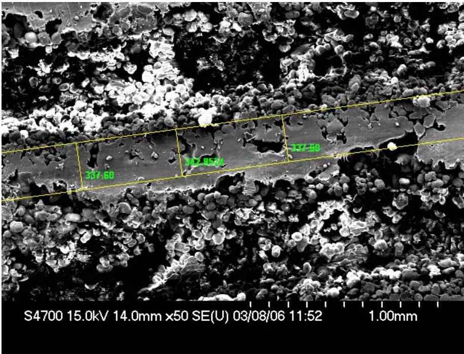
Fig. 5 SEM image of a PA scaffold. The thickness of the strut shown in this image is the distance between the two lines.
