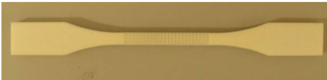
Fig. 2. Specimen used to test the effective modulus of the PA scaffolds in tension
