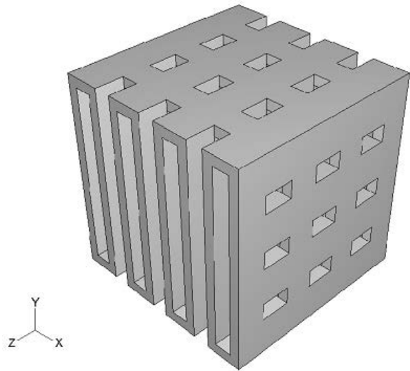
Fig. 6 PA scaffold structure that was modelled.
