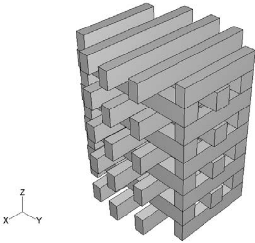
Fig. 7 PCL scaffold structure that was modeled.
