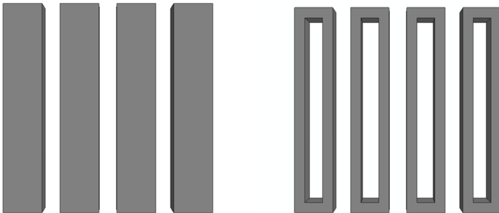
Fig. 1 a) Designed struts, b) this is the result of using the “outline scan” function in the Sinterstation to fabricate the design in Fig. 1a
