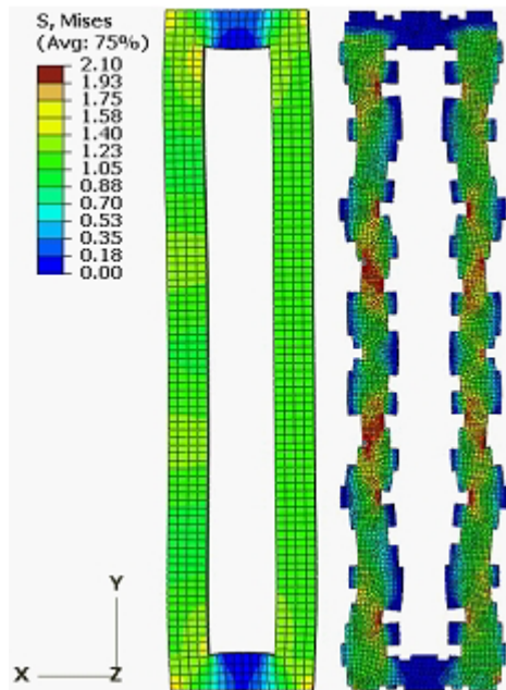
Fig 10. A comparison of stress distributions (MPa) of a smooth strut from Fig 9a and a rough strut from Fig 9b. The rough strut has a greater percentage of elements in violet. These elements contribute little to the scaffold's effective modulus.
