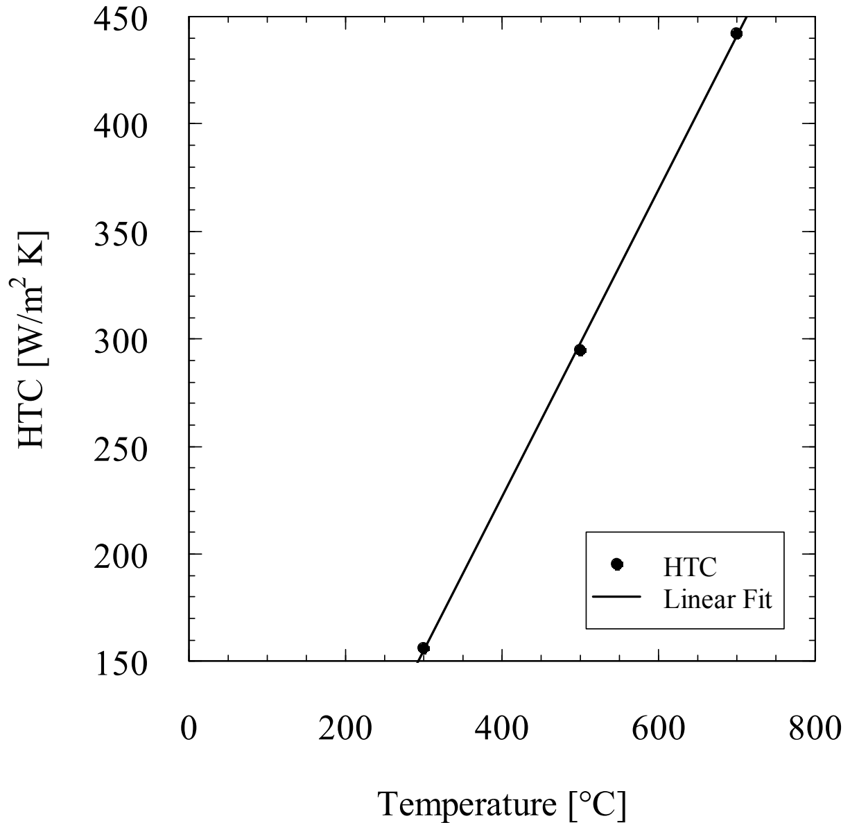
Figure 15: Calculated contact HTC from Gleeble cooling data as a function of temperature
