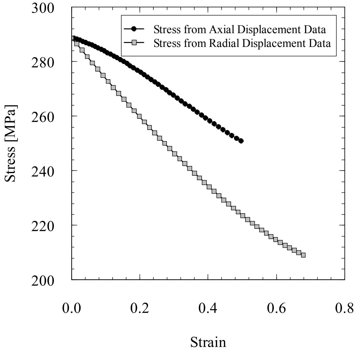
Figure 25: Comparison of stress-strain curves derived from axial and radial displacement measurements ( T=1100^{\circ}\text{C} , \dot{\varepsilon}=1\text{s}^{-1} , m=0 , \eta=0.9 )
