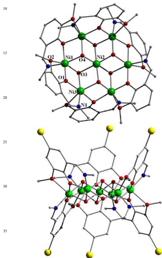
Fig. 1 Molecular structures of complexes 1 (top) and 4 (bottom) viewed perpendicular and parallel to the [Ni_7] plane respectively. Colour code: Ni = green, O = red, N = blue, C = silver, Br = yellow.
