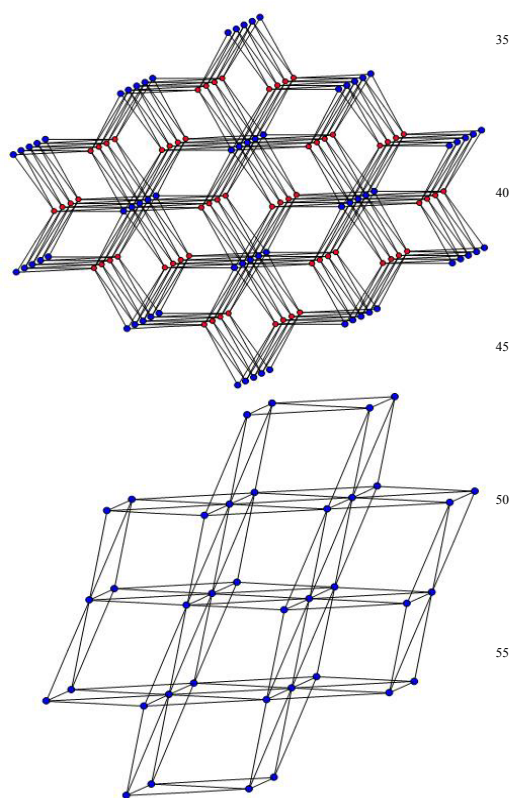
Fig. 4 Crystal packing observed in the crystals of 3 (top) and 4 (bottom) showing the molecular cavities accommodating guest MeNO 2 (red spheres), and MeCN (grey / blue spheres) solvent molecules respectively. NO 3 - counter anions have been omitted for clarity.
