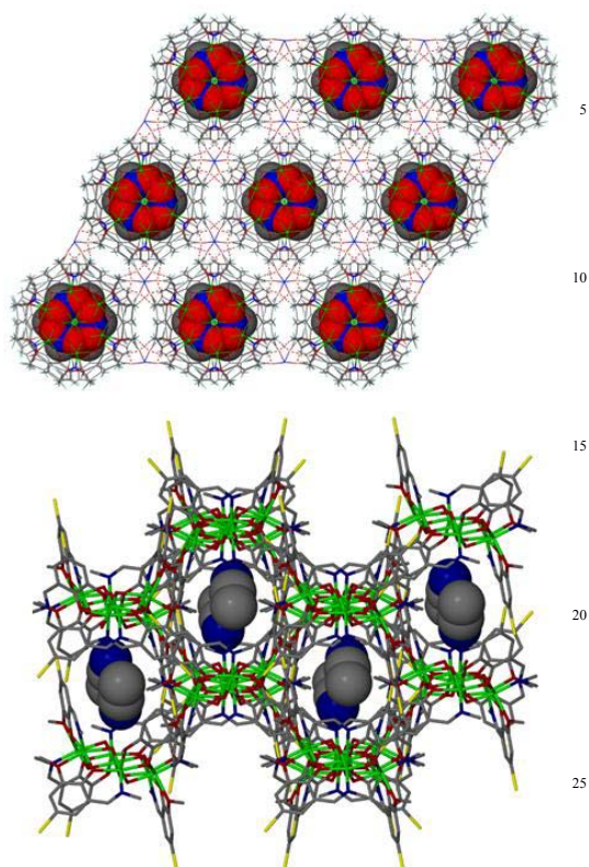
Fig. 4 Crystal packing observed in the crystals of 3 (top) and 4 (bottom) showing the molecular cavities accommodating guest MeNO 2 (red spheres), and MeCN (grey / blue spheres) solvent molecules respectively. NO 3 - counter anions have been omitted for clarity.
