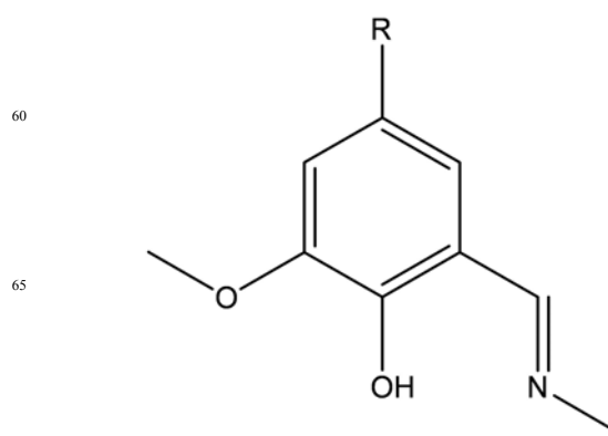
Scheme 1 Structure of the Schiff base ligands HL 1 and HL 2 utilised in this work (R = H (HL 1 ), Br (HL 2 )).
