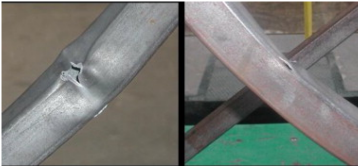
Fig. 11. Fracture damage to brace of Test ST8.
