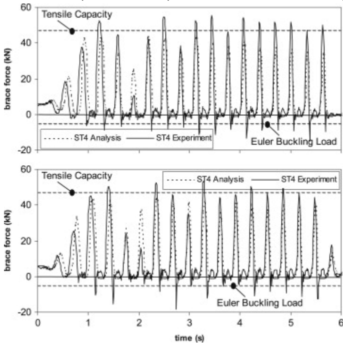
Fig. 9. Experimental and analytical time-histories of brace axial forces during Test ST4.
