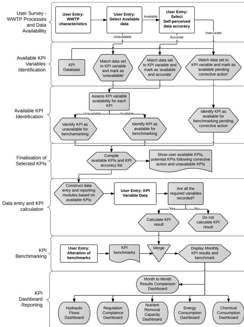
Figure 3. KPICalc framework.
