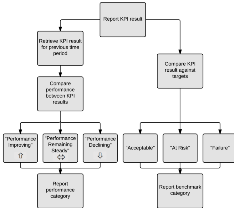
Figure 4. Architecture of the KPI target reporting system
