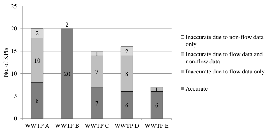
Figure 7. Breakdown of KPI inaccuracies identified by KPICalc
