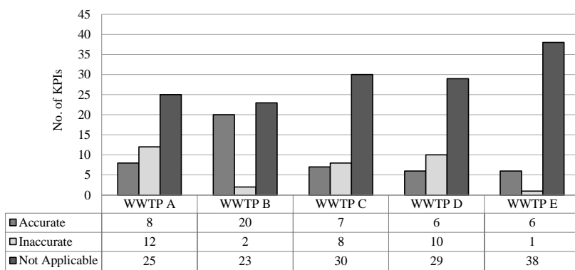
Figure 6. Data availability and accuracy results
