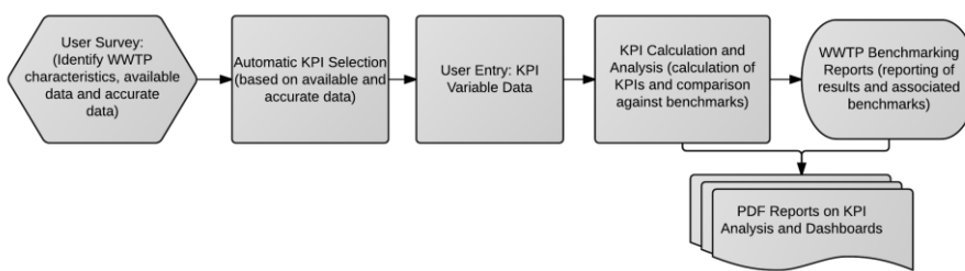
Figure 2. A basic overview of KPICalc.
