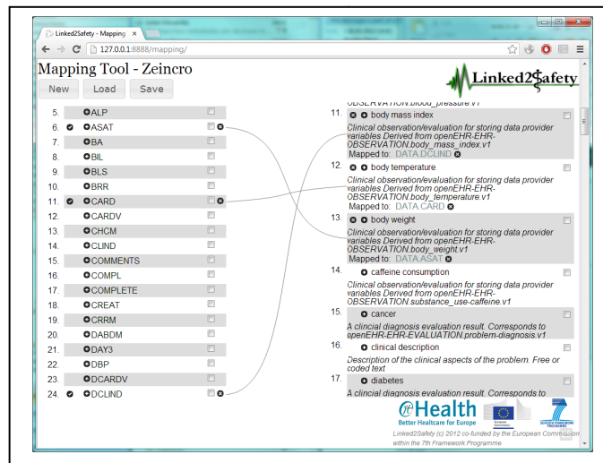
Figure 4. Mapping Tool UI Design
