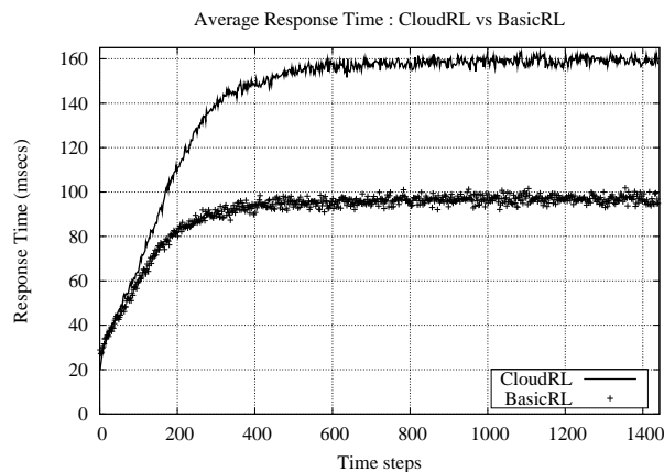
(a) Average Response Time : CloudRL vs BasicRL
