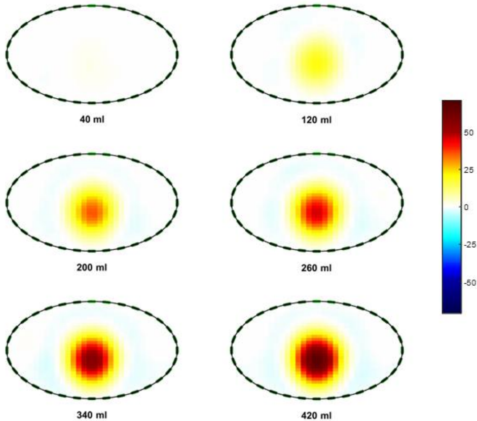
Figure 4.1: Sample images in the 60 dB TC1 dataset of six different bladder volumes. Going across then down, the images correspond to increasing bladder volumes of {40, 120, 200, 260, 340, 420} ml at a urine conductivity of 2 S/m and 60 dB SNR. Spatial changes can be seen with volume change along with a strong contrast between the pixel intensities in the location of the bladder. Note: The colour bar is in arbitrary units and indicates the change in conductivity between the test data and the reference data.
