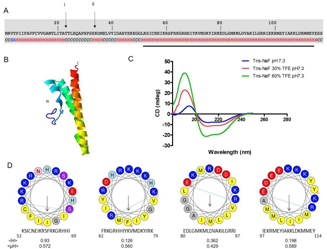
Fig 2. Sm16 predominantly consists of an amphipathic alpha helix. (A) Predictive secondary structure of Sm16 generated using I-TASSER: H—Helix; S—Strand; C—coil. Arrow (i) denotes the SignalP 4.1 predicted cleavage site for an N-terminal secretory signal peptide between residues 22 and 23, and arrow (ii) shows the commencement of the synthetic Sm16 (34–117) peptide sequence. The black line indicates the portion of Sm16 that is amphipathic. (B) 3D model of full length secreted Sm16, generated using I-TASSER (C) Circular dichroism analysis performed on recombinant Sm16 in the absence of tetrafluoroethylene (TFE), in 30% TFE, and 60% TFE. (D) Helical wheel analysis of Sm16 performed using HeliQuest identified four hydrophobic faces (indicated by blue line through helix) in continuous succession in the amphipathic C-terminal helix. <math>\langle H \rangle</math>—Hydrophobicity; <math>\langle \mu H \rangle</math>—Hydrophobic Moment.
