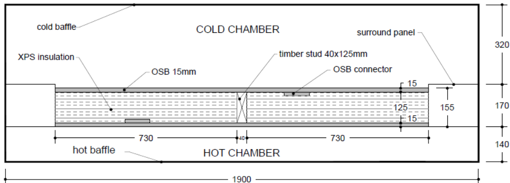
Fig.7. Cross-section of Specimen 3 inserted in hot box.
